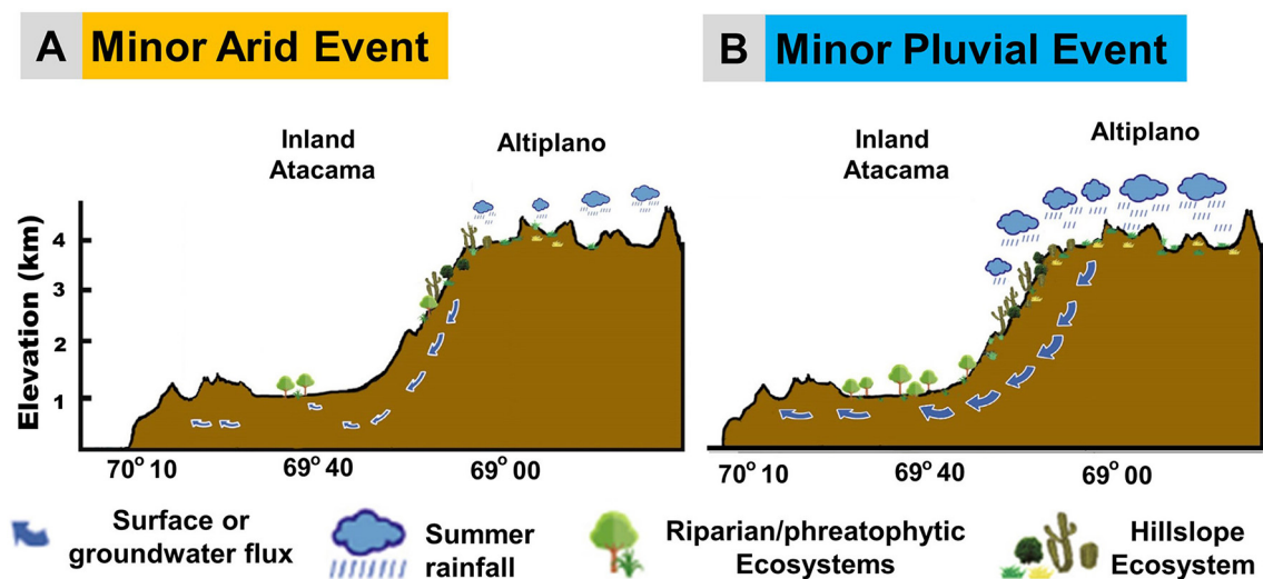
Fig. 2. Schematic illustration contrasting minor climate variations associated with arid and pluvial events in the Chilean Atacama Desert caused by changes in rainfall at altitude. These periods were within an overall arid regime in the Central Depression, and the sketch exaggerates the differences in water and vegetation. See Section 2.2 for details. Figure after Santoro et al. (2017).
