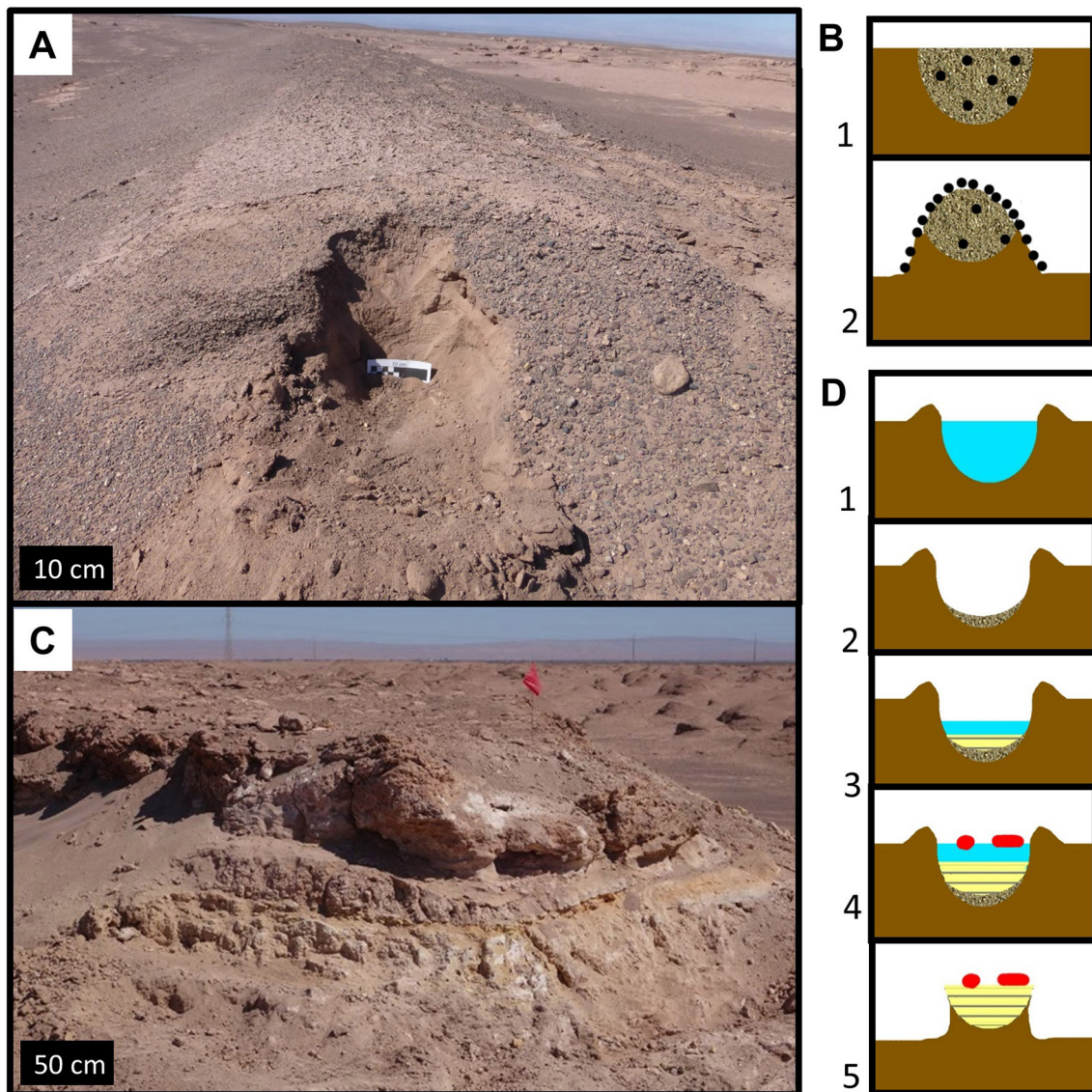
Fig. 17. Comparison of proposed evolutionary sequence for two ridge types at Salar de Llamara, Chile. In both models, the brown layer represents the surrounding materials, presumed to be ancient alluvial/playa deposits. Gravel-capped ridges (A) are interpreted as mudflow deposits with a bimodal grain size distribution (B1) that were deflated by aeolian erosion that removed the finer component and left a residual gravel lag (B2). Sulfate-capped ridges (C) are former sites of a channel (D1) that may have had overbank levees. In panel D, brown corresponds to lower unit, sand texture for channel deposits, yellow for evaporites in upper unit, and red for sulfate plates. Over time, the abandoned channel (D2) was episodically filled with an evaporative sequence (yellow, D3) that formed via groundwater precipitation (possibly ponded) or backed-up surface flow into a lake. At a later time, changes in the chemistry of ponded water facilitated gypsum domes and/or microbial mats (red dots in D4), and their residual are sulfate plates on the surface of the deflated ridge today (D5). Wind erosion stripped the overbank deposits, if any, as well as country rock, resulting in the inverted channel. Surface-conforming halite is found on the flanks of both ridge types and is interpreted to form after topographic inversion took place as a consequence of remobilization of soluble salts.
