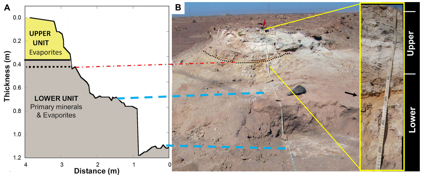
Fig. 14. Simplified stratigraphic section at sulfate capped R4 ridge. A) Transverse relief profile of northeastern edge of ridge R4 (white arrow in Fig. 12A). Ridge R4 is compositionally subdivided into an upper unit comprised of evaporite minerals, and a lower unit with evaporites and primary minerals (Noe Dobrea et al., 2017). Two stair-steps in the profile correspond to anhydrite-rich hardpans (dashed blue lines) that correlate regionally (Supplementary Fig. S3). B) Photograph of trench section of ridge R4. The topographic survey shown in panel A was conducted along tape measure. Dotted black line corresponds to trace of thin, orange layer (dash-dotted red line identifies location in topographic panel in panel A, and black arrow in enlargement). Close-up view of top section (~0.6 m) is presented at far right to illustrate color and textural variations. Shadow from power line diagonally crosses lower portion of outcrop. See Supplementary Table S2 for color descriptions of layers in ridge R4.
