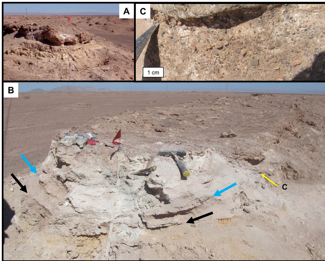
Fig. 13. Some layers in sulfate-capped ridge R4 have concave form. A) Photo taken of brushed ridge R4 outcrop prior to excavation with shovels. Ridge width at top is 1.5 m. B) Post-excavation photo of R4 outcrop. Concave shape is particularly evident in two resistant layer components, with blue arrow marking base of upper unit, and black arrow marking a layer in the lower unit. The distinctive orange layer also has a concave form but is partially covered in this photo; see Figs. 14B and 16C. Yellow arrow points to enlargement in panel C. C) Close-up of gravel lens in a fine-grained sandstone layer at the boundary between the lower and upper units. Polymict fine to medium gravels are subrounded to rounded in shape and interpreted as a pocket of streamflow deposits.
