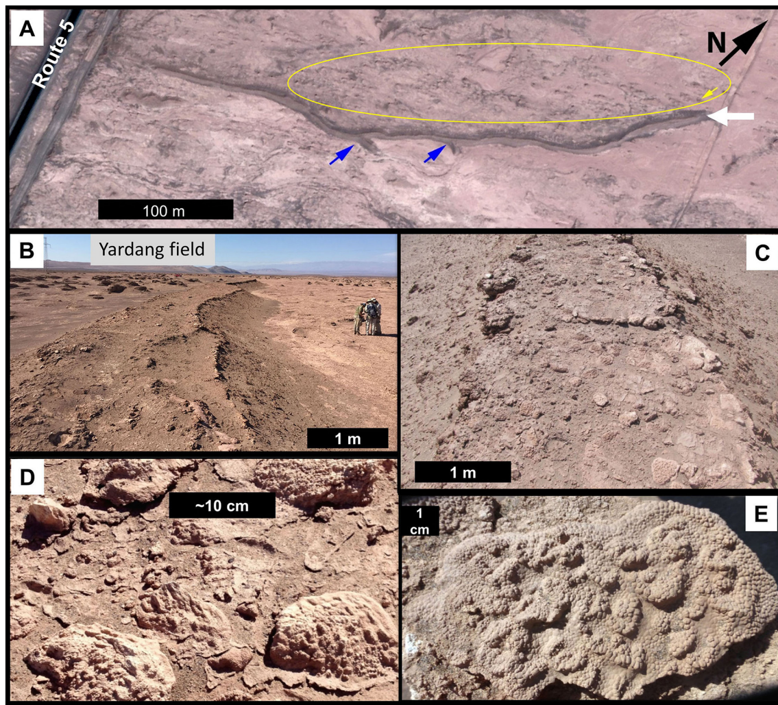
Fig. 12. Examples of sulfate domes and plates associated with sulfate-capped ridge R4. A) Ridge R4 is a relatively linear ridge aligned roughly N30E and has two short spur segments (blue arrows; see also Fig. 3C) in Quickbird image MM128226. A vertical trench was cut at the northeastern edge of ridge R4 (white arrow). Yellow oval outlines a portion of the yardang field (northeast alignment), and the yellow arrow marks location of a nearby yardang where a vertical trench was made (Supplementary Fig. S3). Downfan direction is to the left. B) Perspective upslope view of ridge R4, with rectangular cross-sectional form and concave surface (raised margins) capped by sulfate discs. C) Enlargement of ridge R4 top surface to show the discrete sulfate discs capping the ridge. D) Oblique photograph of gypsum domes and plates on ridge surface. E) Close-up photograph of gypsum plate with bumpy 'goosebump'-like texture.
