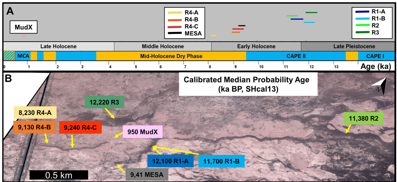
Fig. 15. Summary of radiometric dates for nine wood samples from field site and association with minor paleoclimatic variations. A) Calibrated 2\sigma age range reported per sample relative to geologic epoch and reconstructed climate periods for the Pampa del Tamarugal basin. Periods are color coded to represent minor climatic fluctuations within overall arid conditions, with relatively wet pulses (blue bars), somewhat drier conditions (orange bars) periods, and intermixed wet and arid (patterned blue/orange) during the last 0.5 ka, as reported in Santoro et al. (2017). MCA: Medieval Climate Anomaly. CAPE: Central Andean Pluvial Event. B) Location of sample sites (color legend in panel A insets) are labeled with calibrated median probability age on Quickbird image MM128226. At this scale, some samples are co-located (R1-A & R1-B; R4-A & R4-B). Additional sample details are in Table 1. See Fig. 1B for location of this satellite subscene.
