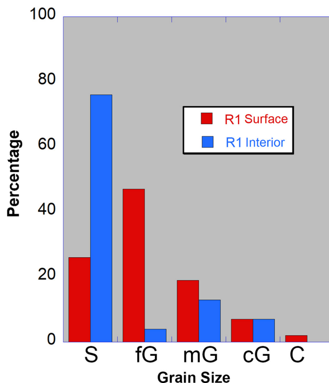
Fig. 10. Histogram of grain size distribution at gravel-capped ridge R1 based on counts over a 0.2 m 2 area with 5 cm grid spacing ( n = 100 ). The percentage of clasts were grouped into sand (S, or finer), fine, medium or coarse gravel (fG, mG, cG), and cobble (C). The size fraction below medium sand was not subdivided. Clasts on the ridge surface (red bars) have a unimodal distribution that is dominantly fine gravel, whereas the interior deposits (blue bars) are bimodal with sand as the dominant grain size and a minor peak at medium gravel. The difference in grain size distribution is attributed to winnowing of fines resulting in a coarser surface deposit.
