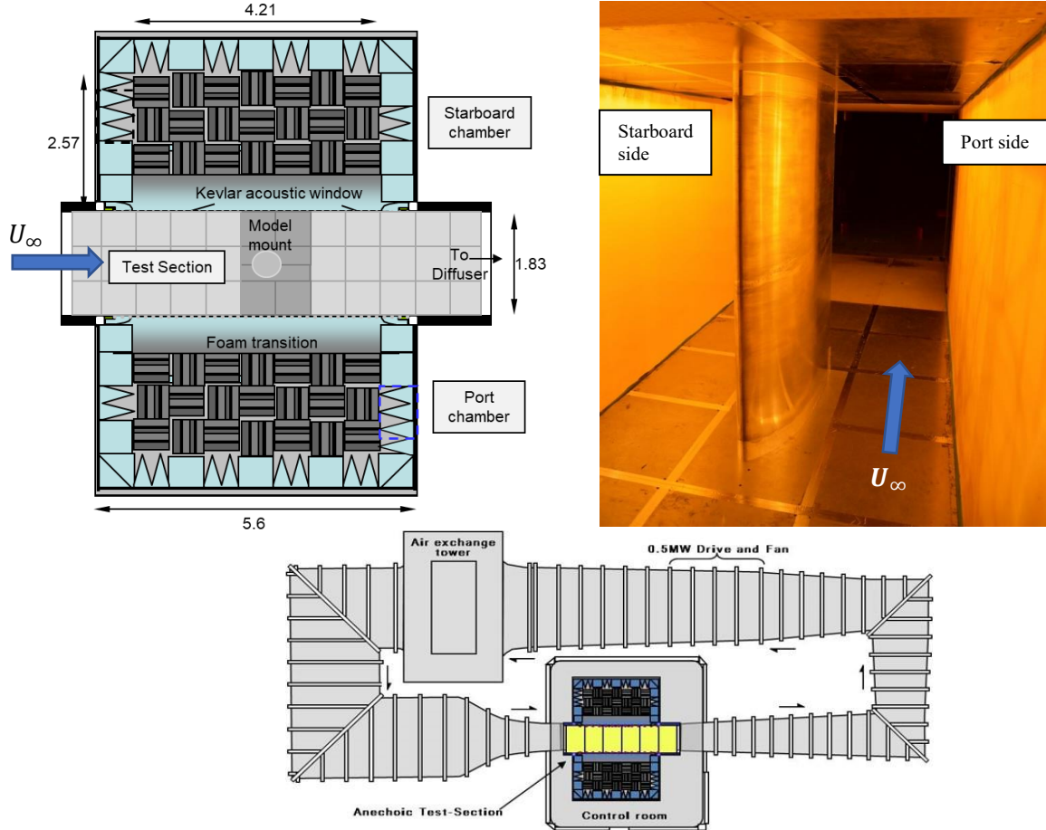
Figure 2. (top left) Cross section through the Kevlar-wall test section and anechoic chambers as seen from above, dimensions in meters, from (Devenport et al. 2013). (top right) View of the DU91-W250 model in the test section as seen from upstream adjacent to the port-side acoustic window. (bottom) The overall view of the Stability Wind Tunnel circuit with the sealed control room including the anechoic chambers and test section highlighted.
