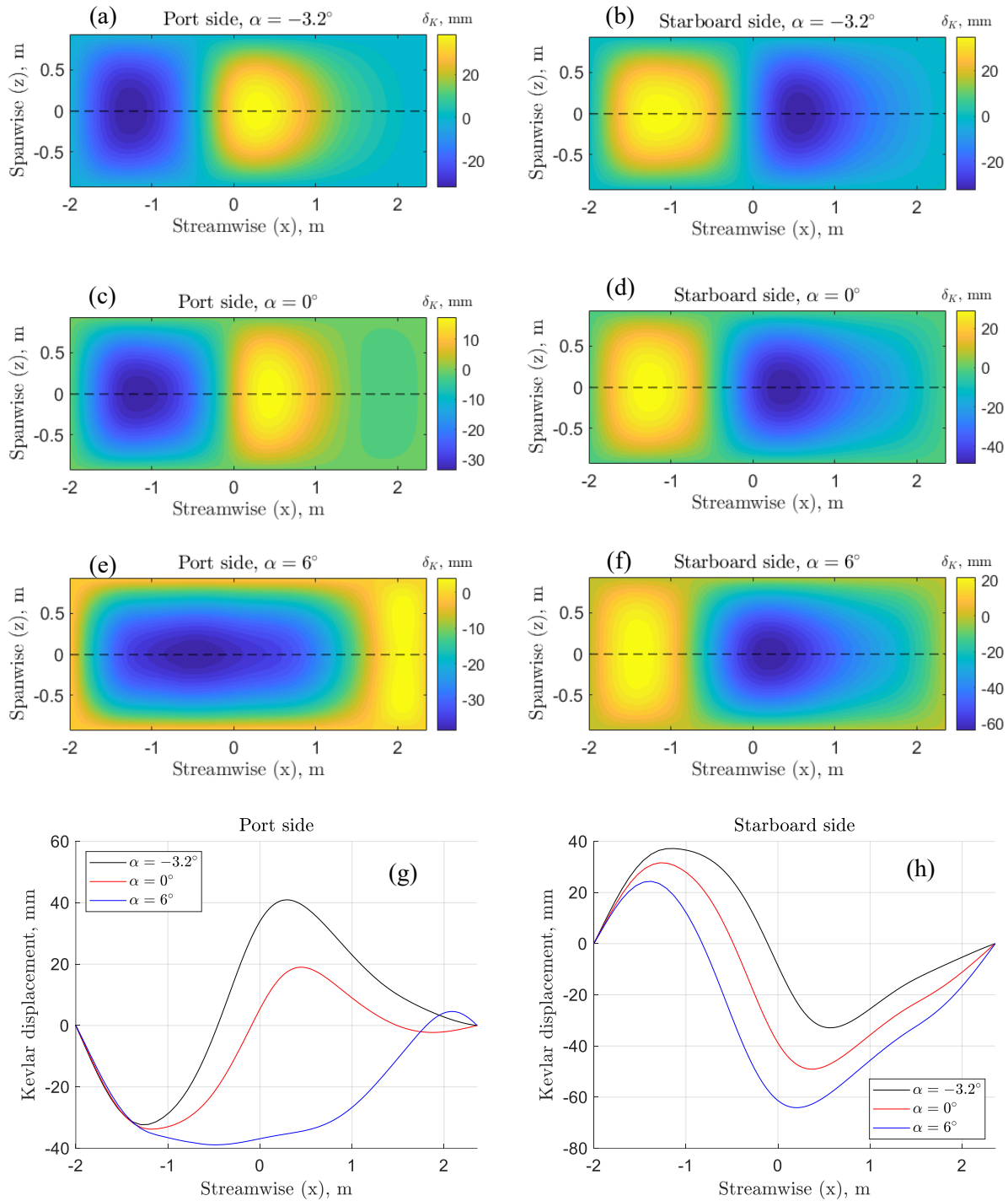
Figure 8. Deflections of the port and starboard side Kevlar windows at \alpha = -3.2^\circ , 0^\circ and 6^\circ , and the deflections of the Kevlar windows across the tunnel mid-span with the mid-span indicated by a dashed line in the contour plots.
