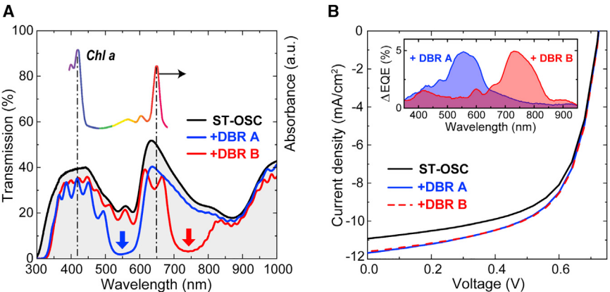
Figure 4. Device characteristics of ST-OSC device with and without DBR coatings (A) Transmission spectra of semi-transparent OSC and the same device combined with DBR-A and DBR-B. Inset is the absorbance of chl a. (B) Current density-voltage characteristics of the ST-OSC along with the ST-OSC with DBR-A and DBR-B. Inset, change in external quantum efficiency ( \Delta EQE) of the ST-OSC with the addition of DBR-A and DBR-B.
