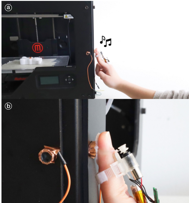
Figure 11: Shows application of (a) adding interactivity to 3D printer, where (b) the screws on the 3D printer feel like soft buttons.
