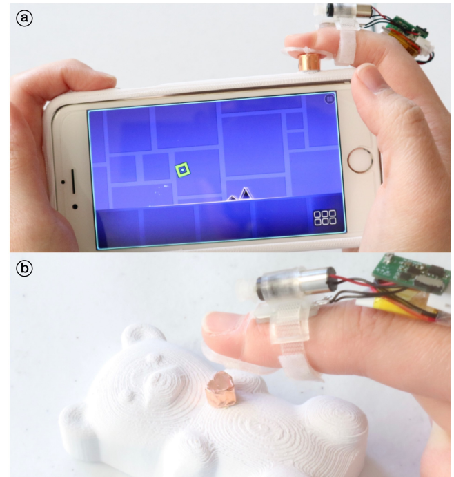
Figure 12: Examples of altering softness of regions on fully rigid 3D printed objects (made from PLA).
