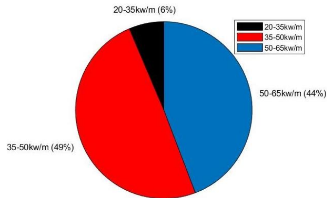
Figure 4. Wave power density hotspot distribution under different thresholds in the Gulf of Mexico (latitude (18°, 30° N), longitude (−98°, −80° W) between 1979 and 2019.
