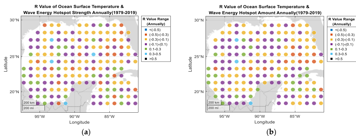
Figure 7. Correlation R values of wave power density hotspots: (a) strengths (20–65 kW/m); and (b) annual amounts and ocean surface temperatures (April 1979–May 2019), within 1^\circ by 1^\circ grids, for the Gulf of Mexico (latitude ( 18^\circ , 30^\circ N), longitude ( -98^\circ , -80^\circ W)).
