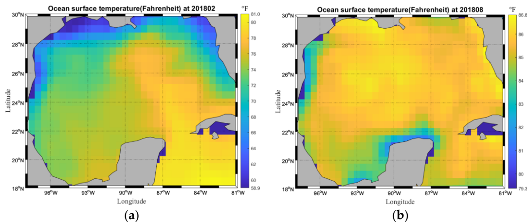
Figure 2. Surface temperature contours in the Gulf of Mexico: (a) February 2018; and (b) August 2018.
