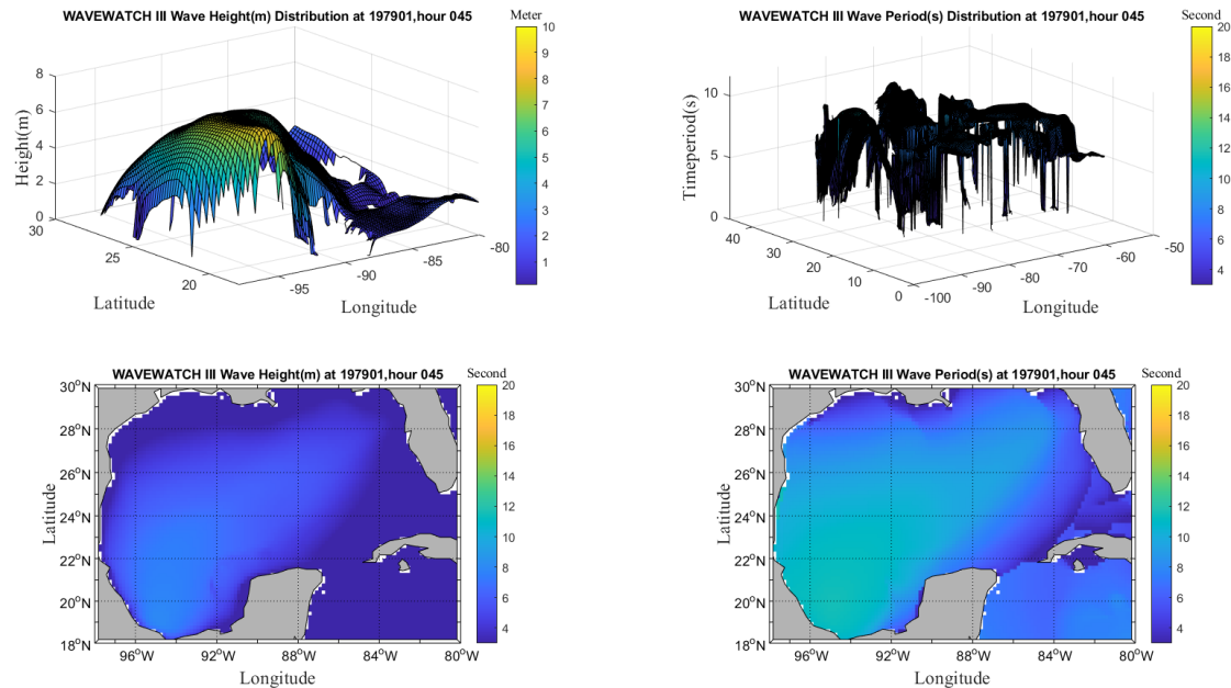
Figure 1. Visualized wave height (m) and wave period (s) distributions, at 3:00 p.m. on 1 January 1979, in different formats.
