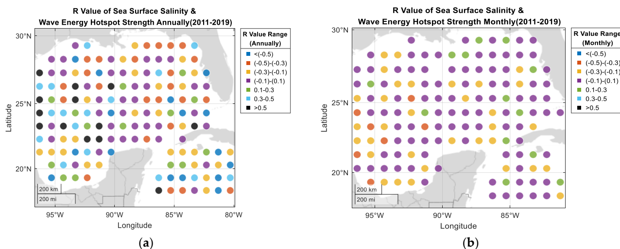
Figure 8. Correlation R values of wave energy density hotspot strengths and sea surface salinities: (a) annually; and (b) monthly (January 2011–May 2019), within 1^\circ by 1^\circ grids, in the Gulf of Mexico (latitude ( 18^\circ , 30^\circ N), longitude ( -98^\circ , -80^\circ W)).
