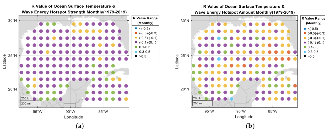
Figure 6. Correlation R values of wave power density hotspots: (a) strengths (20–65 kW/m); and (b) monthly amounts and ocean surface temperatures (April 1979–May 2019), within 1^\circ by 1^\circ grids, in the Gulf of Mexico (latitude ( 18^\circ , 30^\circ N), longitude ( -98^\circ , -80^\circ W)).
