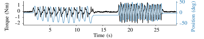
Fig. 6. Torque and position measurements from dynamic backdrive test.
