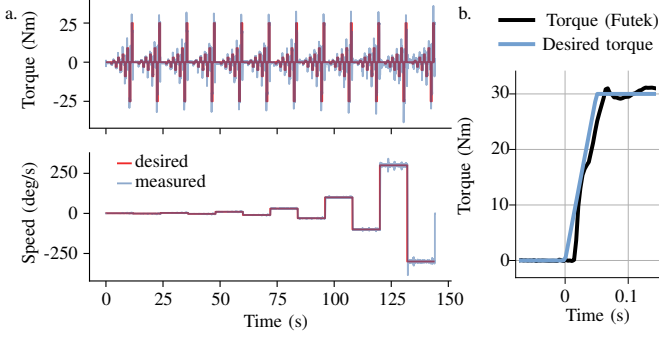
Fig. 7. Constant torque and speed test (a), and 30 Nm step test (b).
