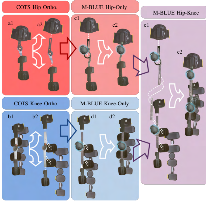
Fig. 3. Modular Backdrivable Lower-limb Unloading Exoskeleton (M-BLUE): a1-2) Commercial off-the-shelf (COTS) T-Scope Hip brace disassembly, b1-2) COTS T-Scope Knee brace disassembly, c1-2) M-BLUE hip-only assembly, d1-2) M-BLUE knee-only assembly, and e1-2) M-BLUE hip-knee assembly.
