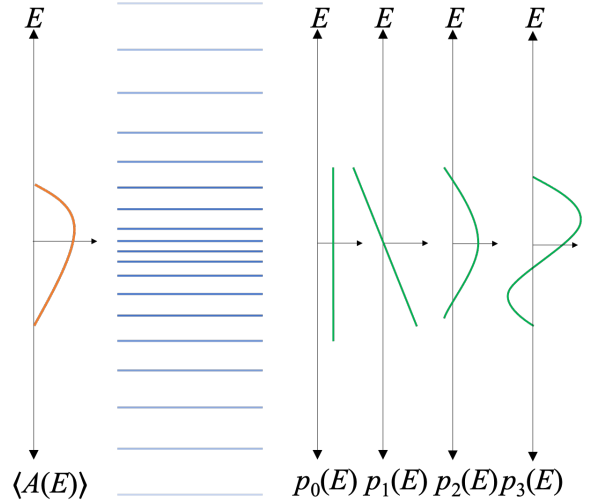
Figure 1. Schematic of the OOPEX philosophy. \langle A(E) \rangle varies slowly with E far from the edges of the spectrum if A satisfies the ETH. p_m(E) are polynomials with m roots, so they oscillate faster with E as m increases. Thus, according to (2), \langle A(E) \rangle receives dominant contributions from small m .
