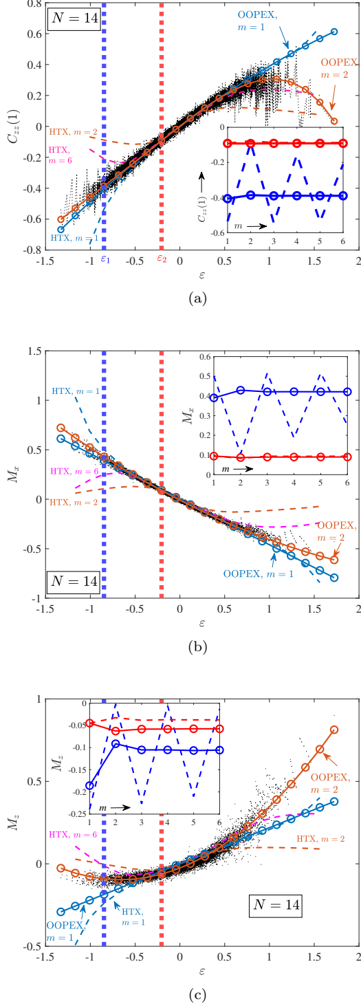
Figure 2. Comparison between computations of (a) C_{zz}(1) , (b) M_x and (c) M_z using OOPEX (solid with markers), ED (dotted) and HTX (dashed) for a N=14 -site chain. OOPEX results for truncation at m=2 agree excellently with ED whereas HTX shows significantly worse agreement even at m=6 . Insets show the truncation order-dependence of the OOPEX and HTX at \epsilon_1 = -0.8475 (blue) and \epsilon_2 = -0.2048 (red) marked in the main figure. The OOPEX converges almost immediately while HTX shows drastically poor convergence away from the middle of the spectrum.
