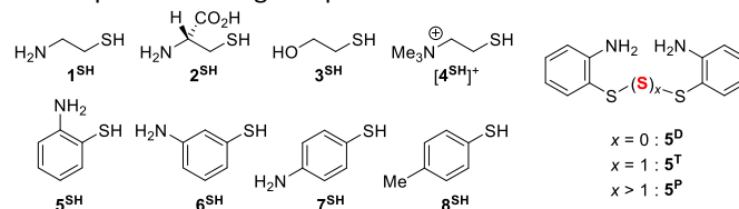
Figure 1. Structures of thiols ( N SH ) studied, along with examples of di(2-aminophenyl) disulfide ( 5 D ), trisulfide ( 5 T ), and higher polysulfides ( 5 P ).
