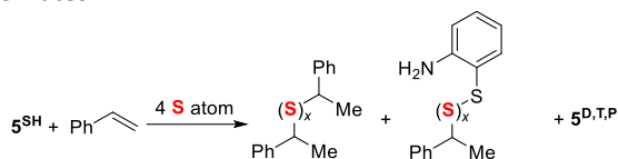
Figure 5. 2-aminothiophenol-mediated addition of sulfur to styrene.
