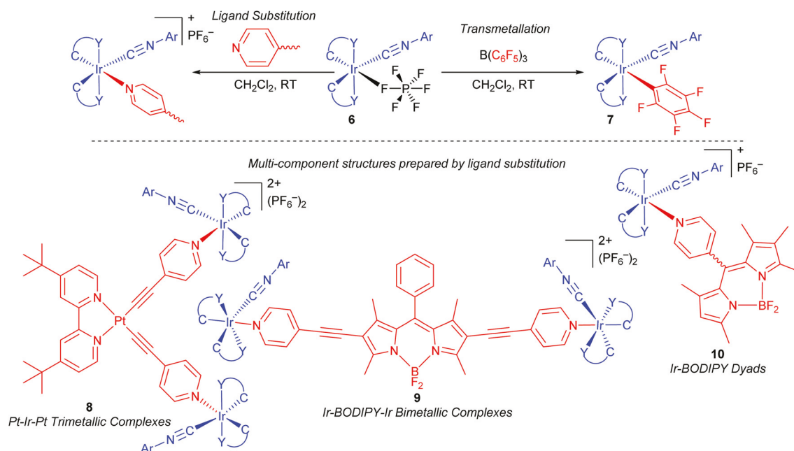
Scheme 3 Reactivity of \text{Ir}(\text{C}^{\wedge}\text{Y})_2(\text{CNAr})(\text{FPF}_5) complexes and their application in the preparation of complexes with multiple photoactive building blocks.
