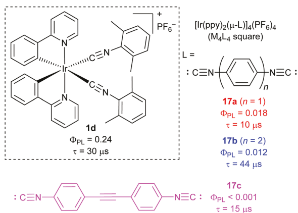
Fig. 8 PL data for a series of [\text{Ir}(\text{ppy})_2(\mu\text{-L})_4](\text{PF}_6)_4 squares as a function of the bridging isocyanide, in comparison to a mononuclear analogue.
