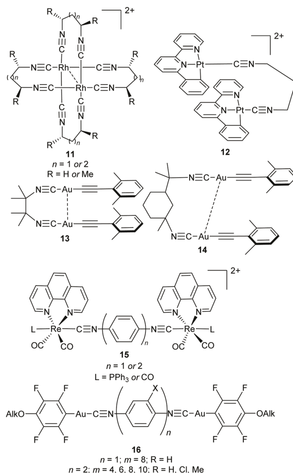
Fig. 6 Structures of dinuclear isocyanide-bridged luminescent complexes.
