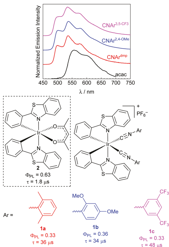
Fig. 4 Summary of photoluminescence data for \text{Ir}(\text{bt})_2(\text{acac}) ( 2 ) and three bis(aryl isocyanide) analogues ( 1a–c ). The spectrum of complex 2 is adapted with permission from ref. 20. Copyright 2001 American Chemical Society.
