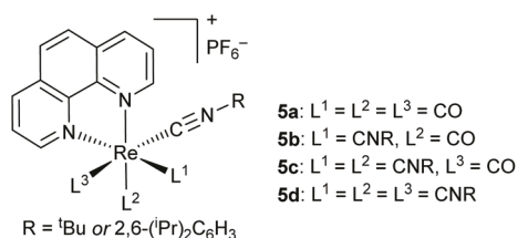
Fig. 5 Structures of luminescent rhenium(i) complexes with ancillary isocyanide ligands.
