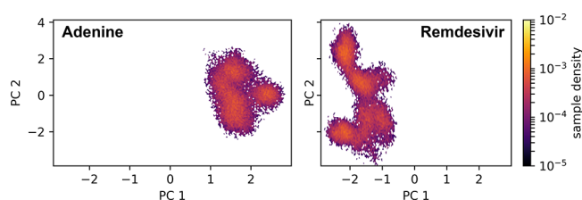
Figure 8. Active site conformational dynamics of the RdRp complex with adenine or remdesivir present. C\alpha distances between active site residues described in the main text have been projected onto the first two principal components (PC1 and PC2). The sample density describes the fraction of simulation time spent in a particular state in PC-space.
