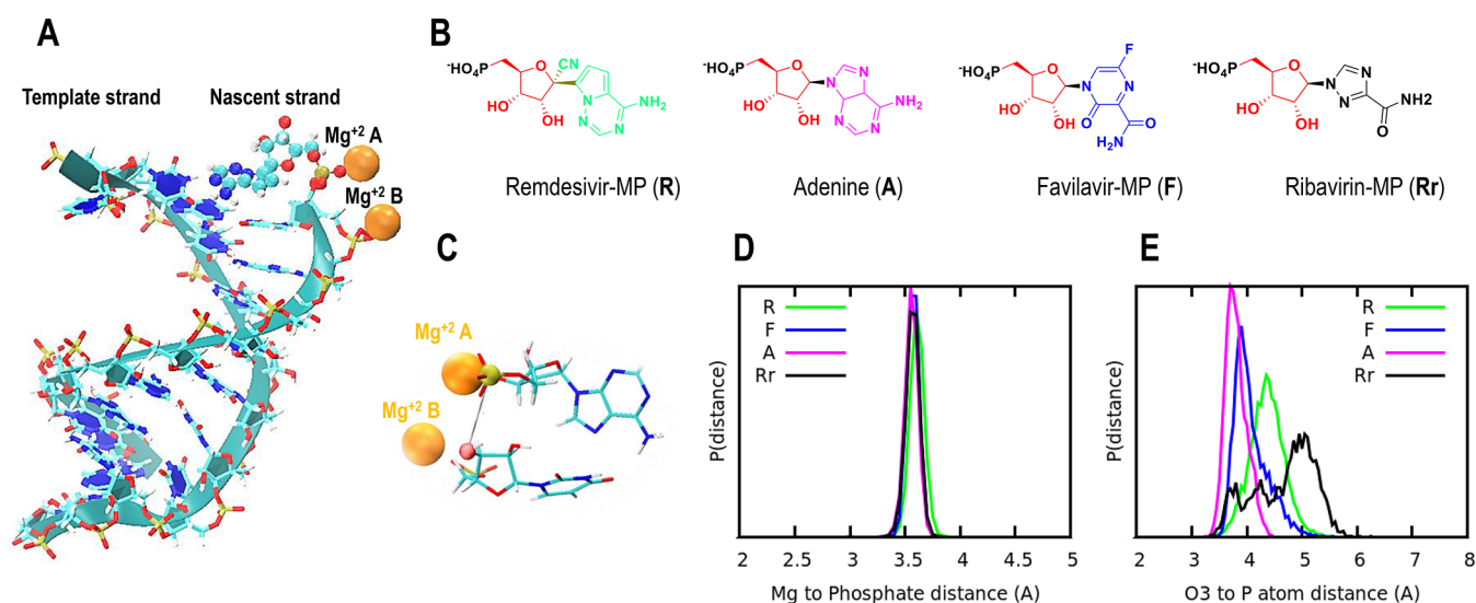
Figure 1. (A) Global structure of the RNA at the nsp12 catalytic site: template and nascent strands are shown in cyan, as well as the Mg 2+ ions in orange. (B) Chemical structure of the monophosphate form of adenine and the other nucleotide analogues studied here. (C) Zooming in at the nsp12 catalytic site: Mg 2+ ions are shown as orange spheres, and the RNA nucleotides are shown as sticks. The last nucleotide in the nascent strand, 3'-end of the RNA chain, is located next to Mg 2+ B, and the nucleotide that is being incorporated to the 3'-end of the nascent RNA strand is located next to Mg 2+ A. The atoms that are subject to further covalent bond formation, phosphorus (P) and oxygen (O3'), are both highlighted as yellow and red spheres, respectively. (D) Probability distribution for the distances between the phosphate group belonging to the monophosphate nucleotide analogues and Mg 2+ A located at the catalytic site. (E) Probability distribution for the distances between phosphorus atom (P) belonging to the phosphate group of the monophosphate analogues and O3' atom of the 3'-terminal nucleotide. In both cases, green, pink, blue, and black are used for remdesivir, adenine, favilavir, and ribavirin, respectively.
