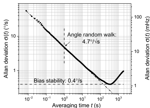
Fig. 4. Diamond gyroscope: Allan deviation. Diamond gyroscope noise measurement as a function of averaging time. The diagonal dash-dotted line shows a 1/\sqrt{t} dependence consistent with a white frequency noise.
