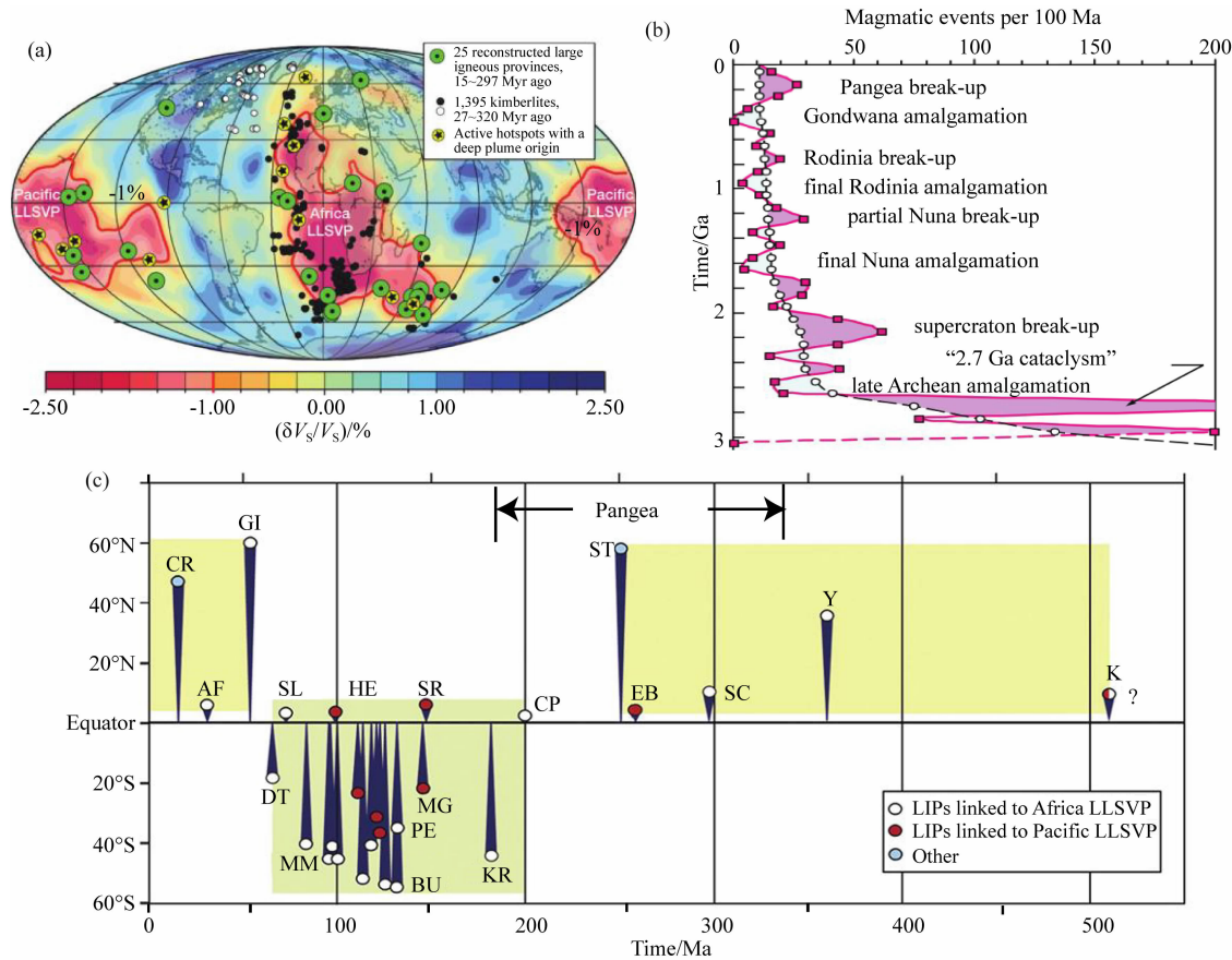
图 4 热点火山、LIP 分布和地幔 S 波波速异常(Becker and Boschi, 2002) (a), 过去 30 亿年的岩浆活动随时间的变化(Ernst and Bleeker, 2010) (b), 及过去 5 亿年的 LIP 随时间的变化(Torsvik et al., 2008a) (c). 图 4b 标示了重要的地质构造事件, 图 4c 还标明了 LIP 的纬度, 及非洲和太平洋 LLSVPs 及 Pangea 的关系 Fig. 4 Distributions of hotspot volcanism, LIP, and S-wave speed anomalies (Becker and Boschi, 2002) (a), temporal variations of magmatism for the last 3 billion years (Ernst and Bleeker, 2010) (b), and temporal dependence of LIP for the last 500 million years (Torsvik et al., 2008a) (c). Fig. 4b also shows major tectonic events, and Fig. 4c marks latitudes of LIP's eruption sites and possible connection of Africa and Pacific LLSVPs with Pangea
