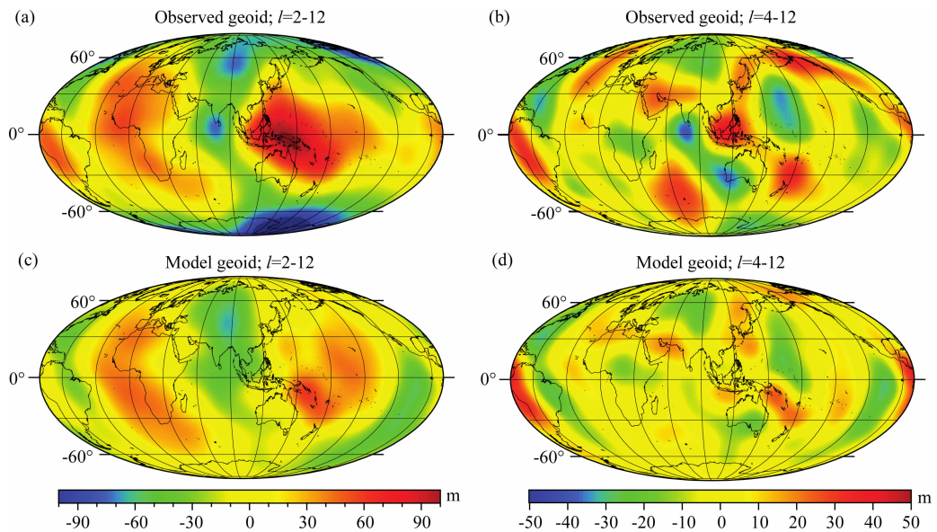
图 3 观测的大地水平面异常:从 2 阶到 12 阶(a)和 4 阶到 12 阶(b). 地幔对流模型计算得到的相应的大地水平面异常(c,d) (Mao and Zhong, 2021a) Fig. 3 The observed geoid anomalies of degrees 2 to 12 (a), and degrees 4 to 12 (b), and the corresponding geoid anomalies from mantle convection model (c,d) (Mao and Zhong, 2021a)
