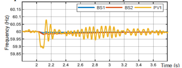
Figure 11. Dynamic frequency outputs with primary-secondary cooperative control
