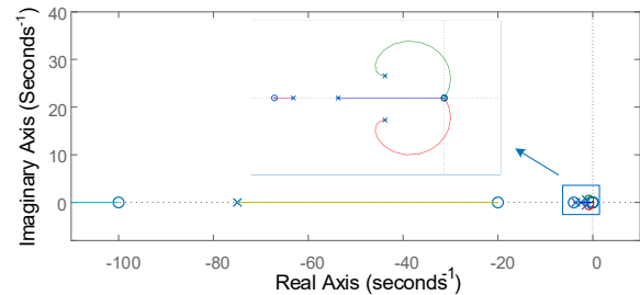
Figure 4. Root locus of the reactive power control loop
