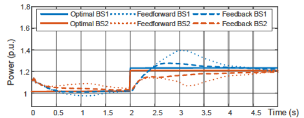
Figure 14. Dynamic power outputs under different control schemes
