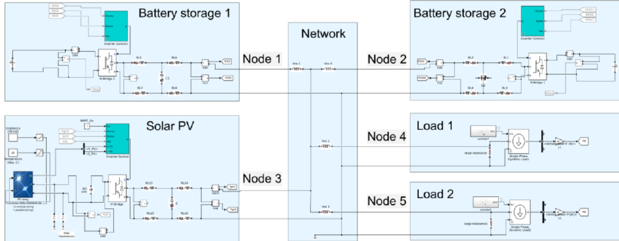
Figure 5. Topology of the residential community microgrid
