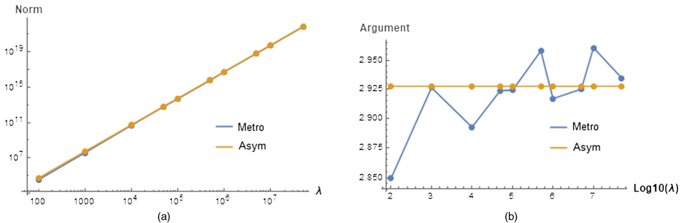
FIG. 7. Absolute values and arguments of G_{14}^{2315} corresponding to different \lambda . The results of the asymptotics are drawn in yellow lines, and the numerical results are indicated by the blue lines.
