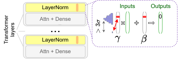
Figure 2: Simplified illustration of our approach to disabling LayerNorm weights. We consistently set the outlier weights \gamma and \beta of the output LayerNorm to zeroes, which results in masking of the corresponding features in the output vectors. We repeat the procedure for all of the Transformer layers of the encoder.
