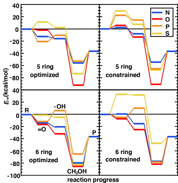
Figure 5. Reaction energetics ( E_{\text{rel}} , in kcal/mol) for the N (in blue), O (in red), P (in orange), and S (in yellow) doped 5- and 6- membered ring graphene model SACs with full geometry optimization (left) or constrained optimization (right). The intermediates are labeled in the bottom left pane: the reactant (R), the oxo intermediate ( =\text{O} ), the hydroxo intermediate ( -\text{OH} ), the methanol-bound intermediate ( \text{CH}_3\text{OH} ), and the product (P). N-doped system in blue, O-doped system in red, P-doped system in orange, S-doped system in yellow, respectively.
