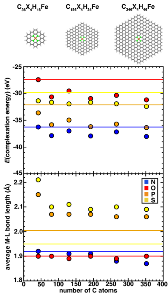
Figure 2. The complexation energy (in eV) and average M–L bond length (in Å) of increasingly large Fe SACs with N, O, P and S-doped graphene flakes. The z-constrained optimization results are shown as the corresponding horizontal lines. Three sizes of representative SACs ( C_{36}X_4H_{16}Fe , C_{186}X_4H_{34}Fe and C_{346}X_4H_{46}Fe ) are shown at top. The structures are shown in stick representation colored as follows: Fe in brown, dopant coordinating atoms in green, C in gray, and H in white. Here, the number of C atoms refers to all atoms in the flake prior to insertion of the vacancy and placement of the dopants and iron.
