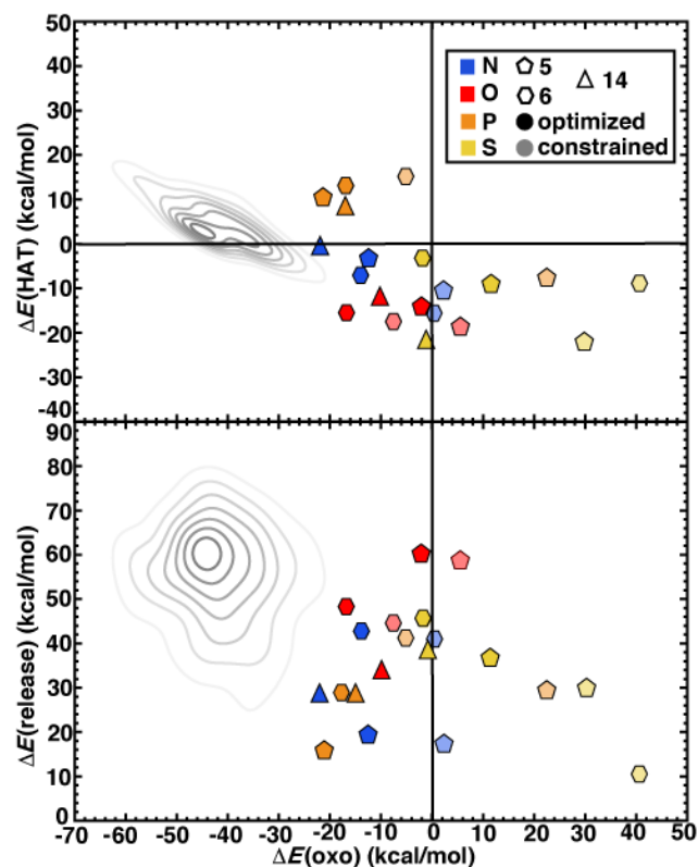
Figure 6. \Delta E(\text{oxo}) vs \Delta E(\text{HAT}) (top) and \Delta E(\text{oxo}) vs \Delta E(\text{release}) (bottom) reaction energies (in kcal/mol) of representative TMCs from prior work 22 compared to 5-membered (pentagons) and 6-membered (hexagons) ring SAC models, and 14-membered macrocyclic Fe complexes
