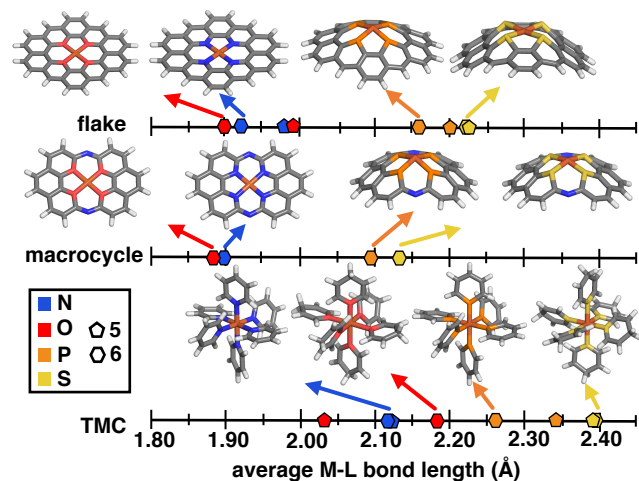
Figure 3. Comparison of Fe-dopant bond lengths between N, O, P and S-doped graphene Fe SAC models (top), 14-membered macrocyclic complexes (middle) and transition-metal complexes (TMCs, bottom). Representative SAC, macrocyclic, and TMC compounds are shown in stick representation colored as follows: Fe in brown, N in blue, O in red, P in orange, S in yellow, C in gray, and H in white. Bond lengths for 5-membered ring complexes and SACs are shown as pentagon symbols and 6-membered ring complexes and SACs are shown as hexagons. Only six-membered ring structures are shown in insets.
