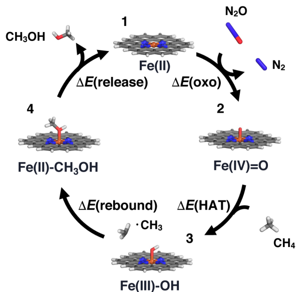
Figure 4. Catalytic cycle for the radical rebound mechanism for conversion of methane to methanol. From the resting state ( 1 , top) in oxidation state II, the cycle proceeds clockwise: iron–oxo ( 2 , right) formation with an N 2 O oxidant, hydrogen atom transfer to form an iron–hydroxo complex ( 3 , bottom), and rebound to form a methanol-bound intermediate ( 4 , left). A representative N-doped 6-membered ring graphene Fe SAC model is shown in stick representation colored as follows: Fe in brown, N in blue, O in red, C in grey, and H in white.
