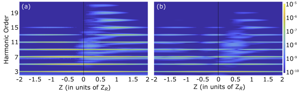
Fig. 1. Comparison of high harmonic radiation spectra as a function of the position of the gas jet along the propagation direction of the driving laser obtained using (a) the Gouy ( g_0 = 0 ) and (b) a short Gaussian pulse phase distribution ( g_0 = -2 ). Note that the propagation distance is scaled in units of the Rayleigh length Z_R = Z_R(\omega_0) . Laser parameters: Peak intensity I_0 = 1.2 \times 10^{14} W/cm 2 , Porras factor g_0 = -2 , central frequency waist at focus W_0 = 30 \mu m, Rayleigh length Z_R = 3534 \mu m. Gas jet parameters: Gaussian distribution of width \sigma = 800 \mu m, peak gas density of 1 \times 10^{18} cm -3 . The vertical black line at Z = 0 is drawn to guide the eye.
