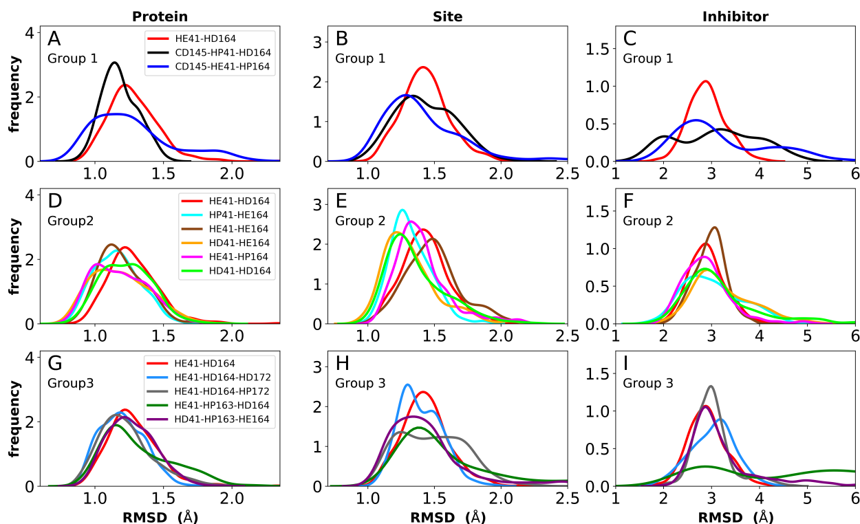
Fig. 8 RMSD distributions for the three protonation state groups from simulations of the ketoamide-bound structure (PDB entry 6Y2G). A-C) RMSD of (A) protein, (B) active site, and (C) inhibitor for Group 1. D-F) RMSD of (D) protein, (E) active site, and (F) inhibitor for Group 2. G-I) RMSD of (G) protein, (H) active site, and (I) inhibitor for Group 3.
