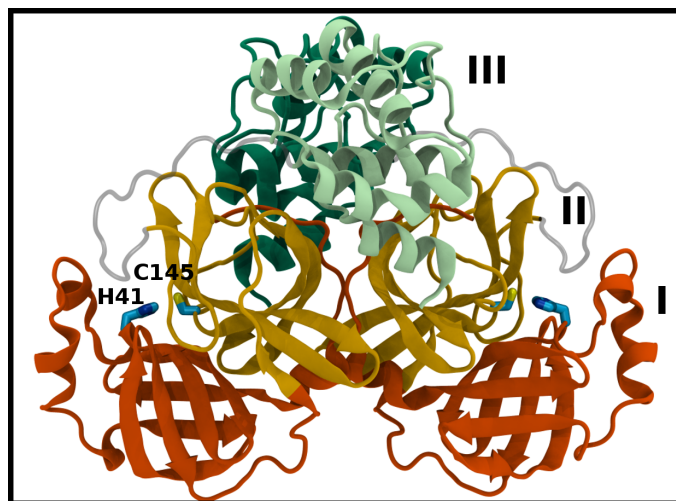
Fig. 1 M Pro dimer structure and binding site interactions (PDB entry 6WQF). M Pro homodimer with the three domains illustrated and color coded as follows: Domain I (dark orange), domain II (gold), and domain III (light green/dark green monomer A/B) with the catalytic dyad residues, His41 and Cys145 (rendered in licorice).
