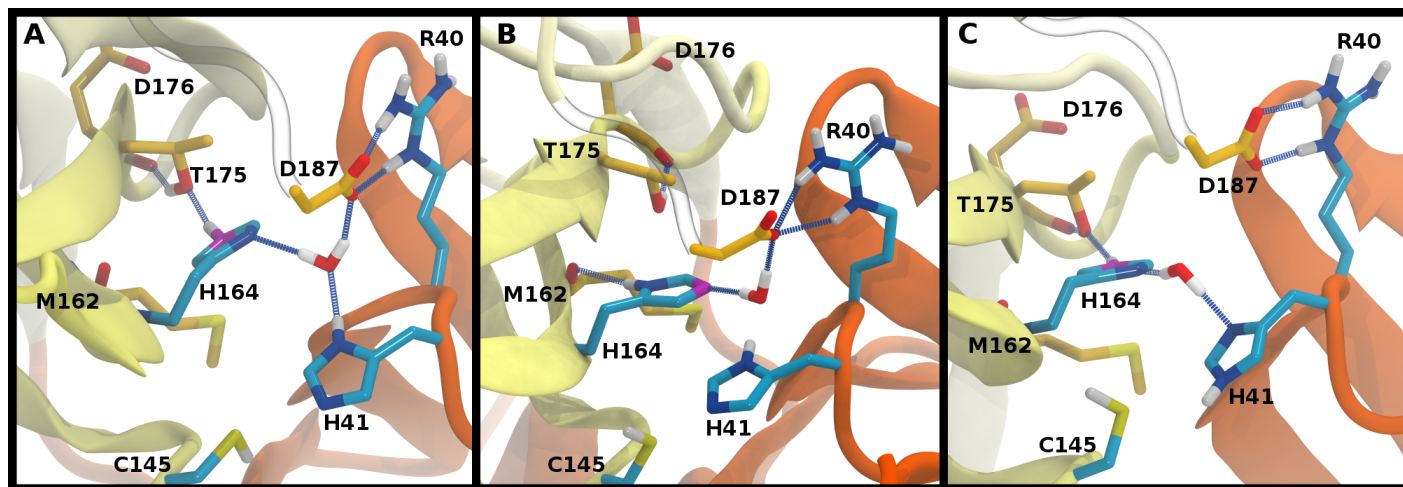
Fig. 5 Hydrogen bonding involving the crystallographic water and His164 local environment. In each image, the NE nitrogen in the His164 side chain is colored magenta. A) HD41-HE164 illustrating hydrogen bond donation from His164 to Thr175. B) HD41-HD164 illustrating the His164 side chain rotation such that a hydrogen bond is formed with the backbone carbonyl of Met162. C) HE41-HE164 illustrating the disruption of the hydrogen bonding interactions and loss of the interaction of the water with Asp187.
