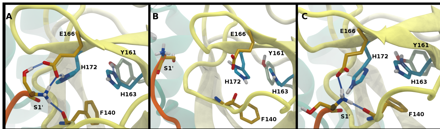
Fig. 4 Hydrogen bonding in the S1 pocket. Example configurations of A) HD41-HE164 characteristic of robust S1 pocket interactions, B) HE41-HD164-HP172 illustrating the rupture of the S1'-Glu166 interaction and loss of the His163-Tyr161 hydrogen bond, and C) HE41-HP163-HD164 depicting the loss of the Tyr161 hydrogen bond donation and the His172-Glu166 interaction.
