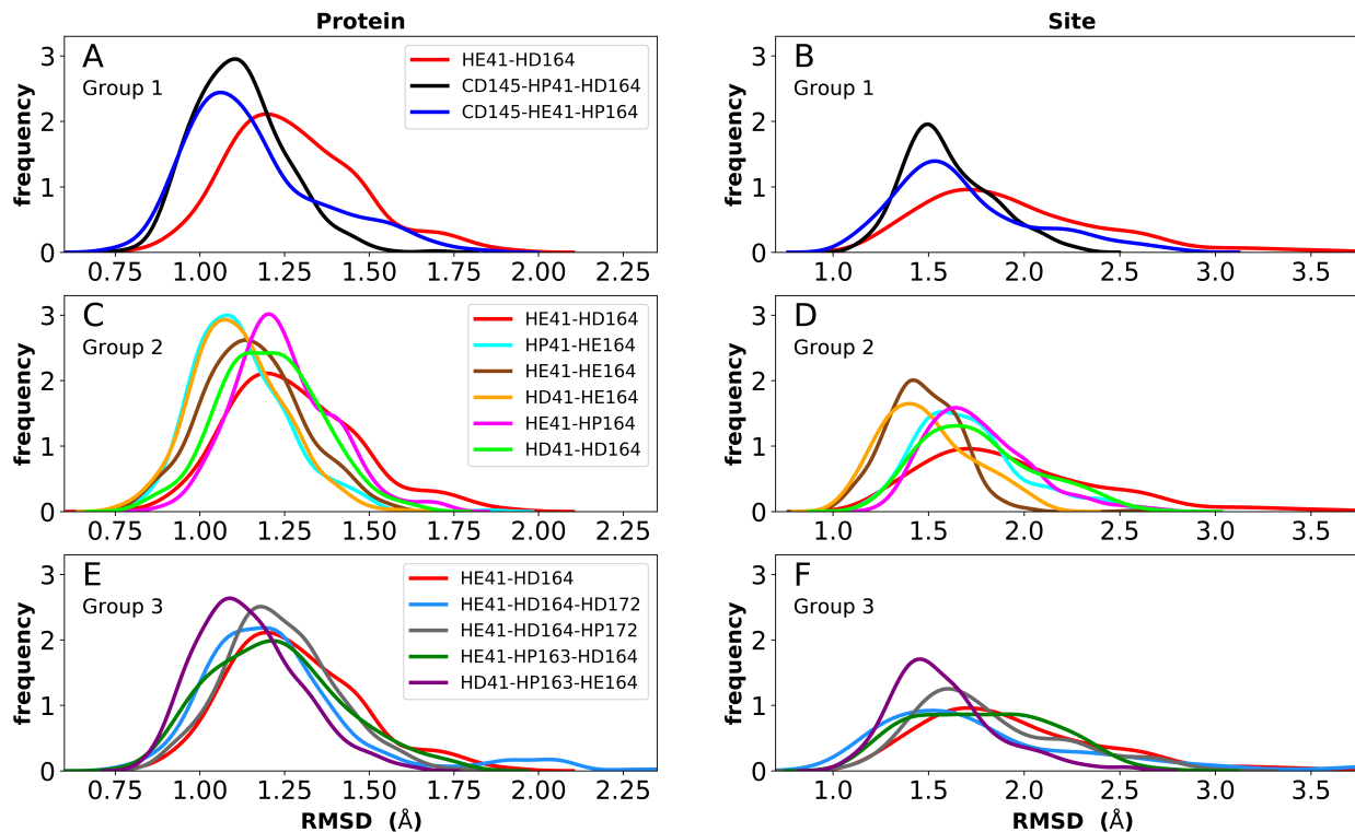
Fig. 3 RMSD distributions for the three protonation-state groups from simulations of the apo structure (PDB entry 6WQF 11 ). A-B) RMSD of (A) protein and (B) active site for Group 1. C-D) RMSD of (C) protein and (D) active site for Group 2. E-F) RMSD of (E) protein and (F) active site for Group 3.
