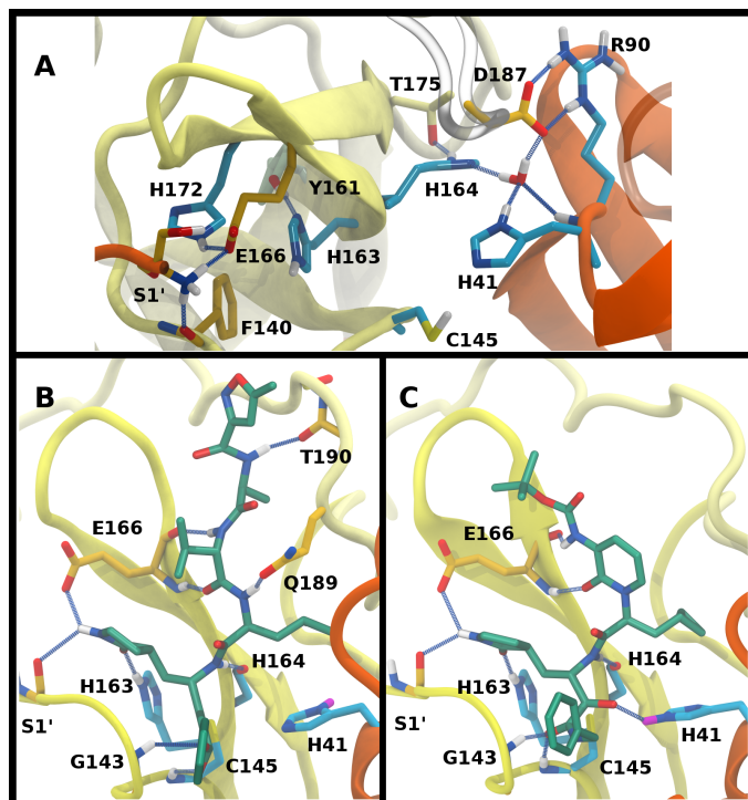
Fig. 2 Hydrogen bonding interactions in the catalytic site for the apo, N3-bound, and ketoamide-bound structures. A) Illustrated for the HD41-HE164 apo state taken from the simulation are the i) catalytic dyad, ii) the crystallographic water bridging His41, His164, and Asp187 as well as His164 with Thr175, and iii) S1 pocket interactions. The N-terminal serine residue is labeled with a prime to indicate that it is from the alternate monomer. B) Binding pocket of N3-bound M pro with hydrogen bonds displayed taken from the HD41-HE164 state. C) Binding pocket of ketoamide-bound M pro with hydrogen bonds displayed, taken from the HE41-HD164 state. The ligands in both B) and C) are rendered in licorice with carbon atoms in green. Note, the His41 hydrogens in the ligand-bound HD41/HE41 states are rendered in magenta, highlighting the alternate protonation for the N3 and ketoamide-bound non-covalent complex with the His164 side chain and water removed for clarity. Hydrogen bonds are illustrated with blue lines.
