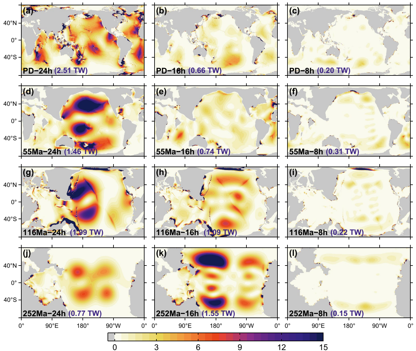
Figure 3. As in Figure 2, but for M 2 energy dissipation rate maps (mW m -2 ). Numbers given in parentheses at the bottom of each subplot present the globally integrated M 2 ocean tidal dissipation rate (TW) of each simulation. Results for T = 24 hr (leftmost panels) can be compared with Green et al. (2017), who found total ocean tide dissipation rates of (1.44, 2.12, 0.90) TW for the three paleo geometries, using another ocean model with a different treatment of self-attraction and loading and wave drag.
