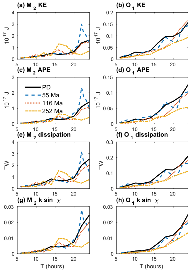
Figure 4. Globally integrated kinetic energy (KE; a and b), available potential energy (APE; c and d), energy dissipation rate (e and f), and k \sin \chi values (g and h), for M_2 (left-hand side subplots) and O_1 (right-hand side subplots) ocean tide simulations with different values of T in Equation 6, and the four bathymetries shown in Figure 1. Four additional T values were used in the 55 Ma simulations, in order to better resolve the peak near 22 hr. Globally integrated KE and APE values are computed via Equation 13. This figure, and all subsequent figures, have legends, and the legends are not enclosed by boxes.
