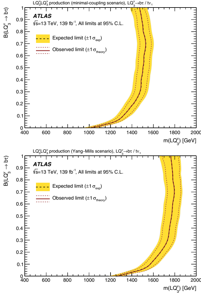
FIG. 10. Expected and observed exclusion contours at the 95% confidence level (C.L.) for the third-generation vector-leptoquark signal model, as a function of the mass m(\text{LQ}_3^v) and the branching fraction B(\text{LQ}_3^v \rightarrow b\tau) into a quark and a charged lepton. The top plot shows the exclusion contour for the minimal-coupling scenario, the bottom plot the exclusion contour for vector leptoquarks in the Yang-Mills scenario. The limits are derived from the binned single-tau signal region.
