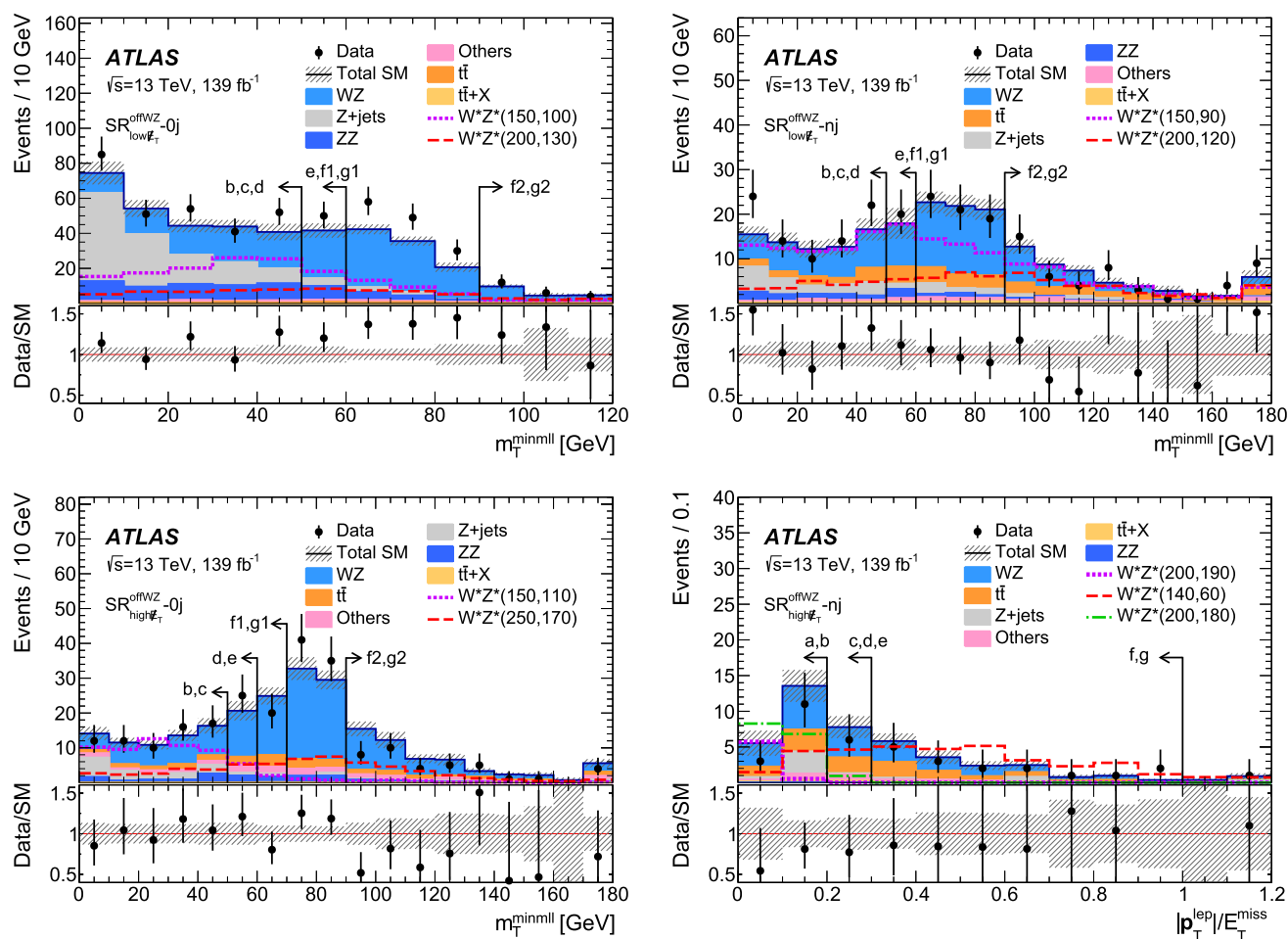
Fig. 14 Kinematic distributions after the background-only fit showing the data and the post-fit expected background, in SRs of the off-shell WZ selection. The figure shows the m_T^{\text{min}} distribution in (top left) \text{SR}_{\text{low}E_T}^{\text{offFWZ}-0j} , (top right) \text{SR}_{\text{low}E_T}^{\text{offFWZ}-nj} and (bottom left) \text{SR}_{\text{high}E_T}^{\text{offFWZ}-0j} , and the |p_T^{\text{lep}}|/E_T^{\text{miss}} distribution in (bottom right) \text{SR}_{\text{high}E_T}^{\text{offFWZ}-nj} . The contributing m_T^{\text{min}} mass bins within each \text{SR}_{\text{offFWZ}} category are summed. The SR selections are applied for each distribution, except for the vari-
