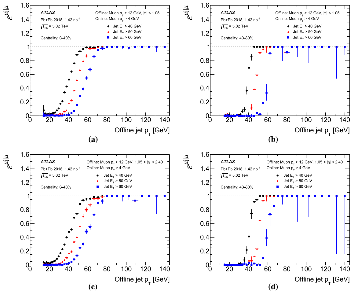
Fig. 16 The conditional muon-jet trigger efficiency, \varepsilon^{\mu j|\mu} , as defined in Eq. (1), as a function of offline jet p_T . The muon-jet triggers shown require a muon with p_T > 4 GeV and jet E_T thresholds of 40, 50, and 60 GeV. The muon-jet trigger efficiency is estimated relative to the single-muon trigger requiring a muon with p_T > 4 GeV. Events are also
