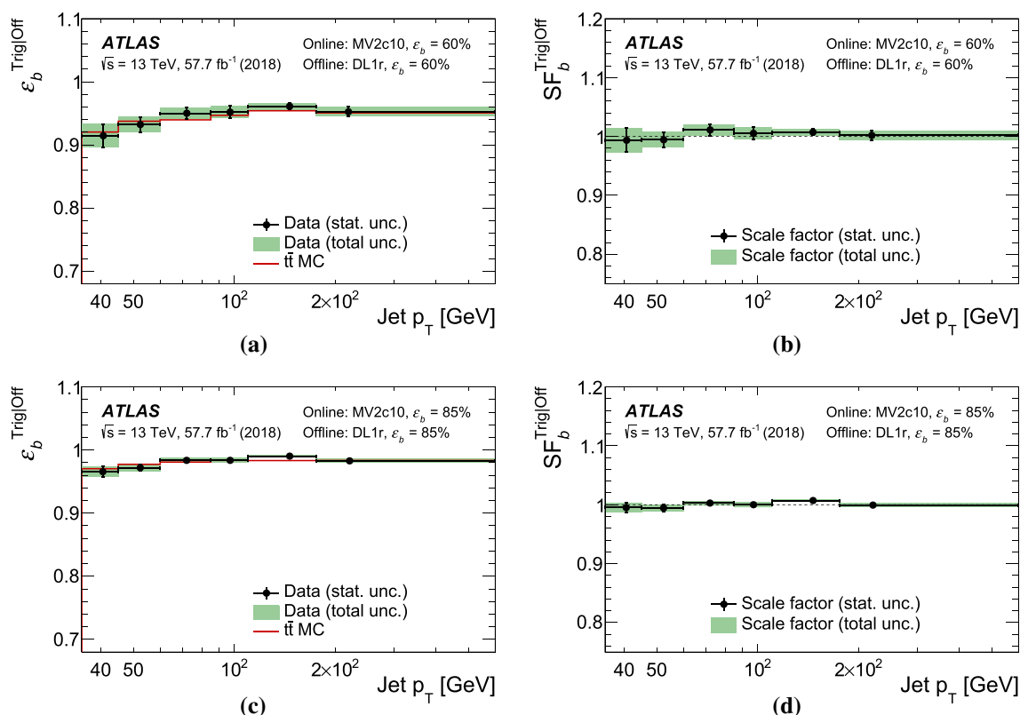
Fig. 14 The conditional b -tagging efficiency, \varepsilon_b^{\text{TrigOff}} , (a, c) and corresponding scale factor, SF_b^{\text{TrigOff}} , (b, d) for the online MV2c10 algorithm for the 60% efficiency working point (a, b) and the 85% efficiency working point (c, d) as measured in 2018 data. Offline jets are required
