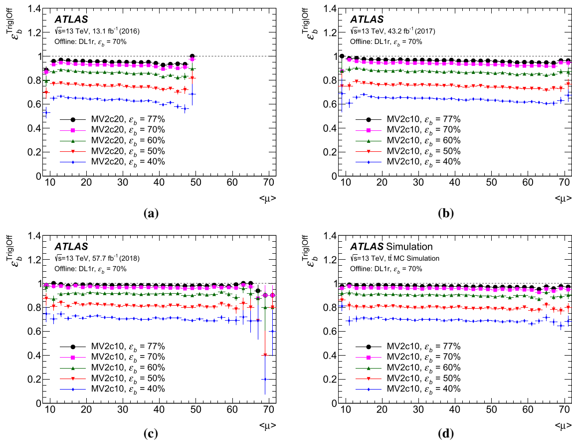
Fig. 15 The conditional b -tagging efficiency, \varepsilon_b^{\text{Trig/Off}} , for data taken in a 2016, b 2017, c 2018, and d simulated t\bar{t} events, as a function of pile-up, \langle\mu\rangle . All working points of the MV2 b -tagging algorithm used
