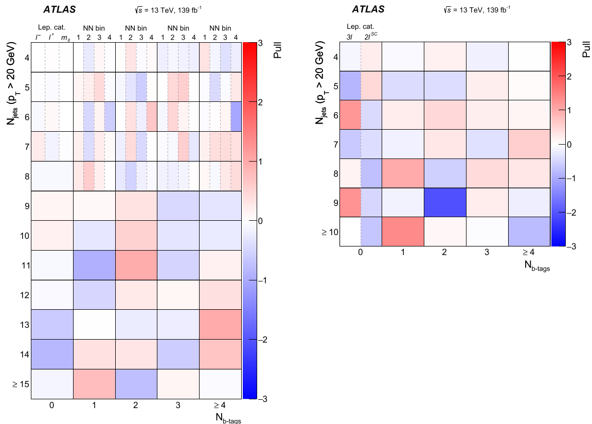
Fig. 7 The observed pulls in all the regions considered in the EWK analysis, in the 1 \ell category (left) and the 2 \ell^{\text{sc}} category (right). The pull is defined as the difference between the observed number of events and the total expected number of events determined by the fit divided by the
