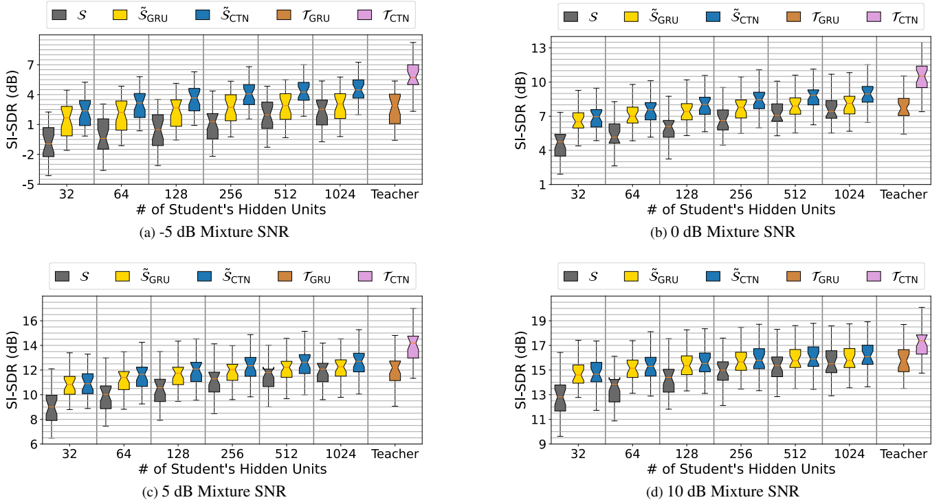
Figure 2: Comparison of SE performances from pre-trained generalists against personalized specialists under various mixture SNR levels. Student models are initialized as 2-layered GRU generalists. Teacher models are provided as references.
