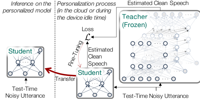
Figure 1: An overview of the proposed KD-based PSE process. The estimated clean speech by the student model is compared against the result from a larger teacher model, whose discrepancy is used to fine-tune the student model. This can be done during the test time as it does not require the clean speech target.
