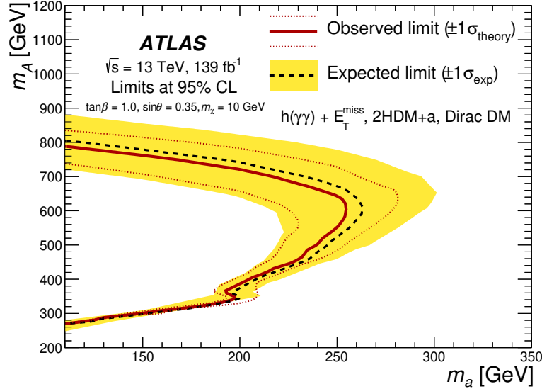
Figure 10. The observed (solid line) and expected (dashed lines) exclusion limit contours at 95% CL for the 2HDM+a model in the m_A - m_a plane, for \tan\beta = 1.0 , \sin\theta = 0.35 , and m_\chi = 10 GeV. The dotted lines represent the \pm 1\sigma theoretical uncertainty for the observed limit. The \pm 1\sigma expected exclusion limit contour is shown as the yellow band. Around the threshold m_A = 350 GeV, the competition between the resonant decay A \rightarrow t\bar{t} and A \rightarrow ah causes the A \rightarrow ah branching ratio to decrease suddenly with a limited increase of m_A , resulting in the feature near m_a = 200 GeV. Above m_A = 350 GeV, the limit is mainly driven by the increased selection efficiency due to the harder signal E_T^{\text{miss}} distribution.
