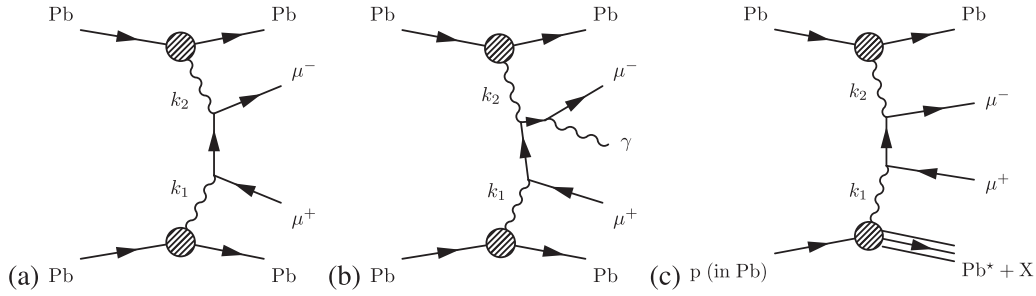
FIG. 1. Diagrams for the (a) leading-order \text{PbPb}(\gamma\gamma) \rightarrow \mu^+\mu^- ( \text{PbPb} ) and (b) next-to-leading-order \text{PbPb}(\gamma\gamma) \rightarrow \mu^+\mu^- + \gamma ( \text{PbPb} ) (middle) Breit-Wheeler process in \text{Pb}+\text{Pb} collisions, and (c) the dissociative \text{PbPb}(\gamma\gamma^*) \rightarrow \mu^+\mu^- + X ( \text{Pb}^*\text{Pb} ) process where one photon is emitted from the substructure of one of the nucleons, leading to nucleon fragmentation in the far-forward direction.
