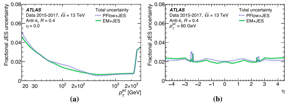
Fig. 24 Fractional jet energy scale systematic uncertainty summed across all components for anti- k_t R = 0.4 jets a as a function of jet p_T at \eta = 0 and b as a function of \eta at p_T = 60 GeV. The total uncertainty is shown for both EMtopo and PFlow jets. Contributions from topology-dependent components are calculated assuming a dijet flavour composition
