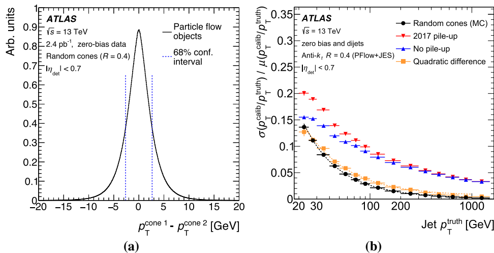
Fig. 27 a The difference in the random cone sums, \Delta p_T^{\text{RC}} , measured in the central region ( |\eta_{\text{det}}| < 0.7 ) in randomly triggered data using PFlow objects. b Comparison between the pile-up noise term N^{\text{PU}} determined using the random cone method (black solid circles) and the expectation
