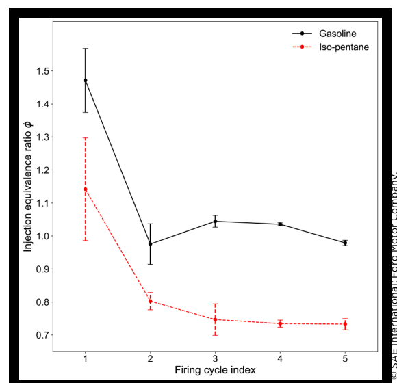
FIGURE 9 Average injection equivalence ratio for firing cycles 1 to 5
