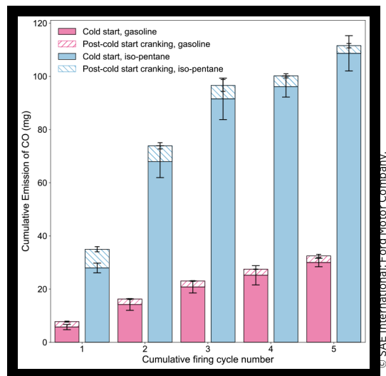
FIGURE 8 Cumulative CO emissions at 1 to 5 firing cycles
