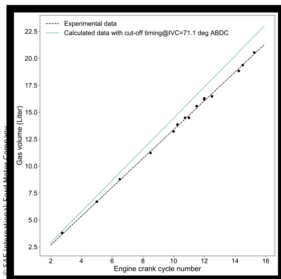
FIGURE 5 Experiment obtained gas volume versus theoretic calculation results
