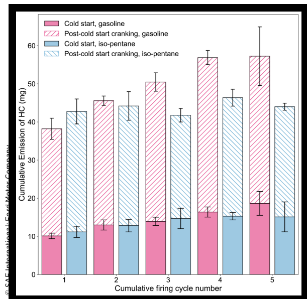
FIGURE 6 Cumulative HC emissions at 1 to 5 firing cycles
