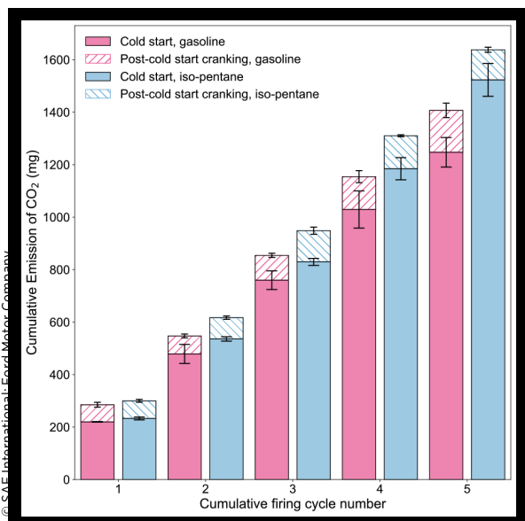
FIGURE 10 Cumulative CO 2 emissions at firing cycles 1 to 5
