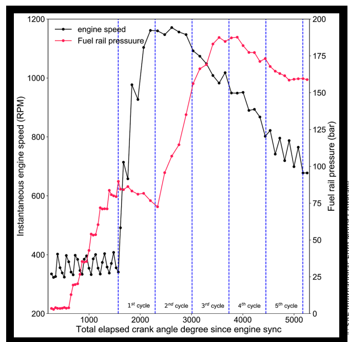
FIGURE 4 Instantaneous engine speed and fuel rail pressure change during cold start
