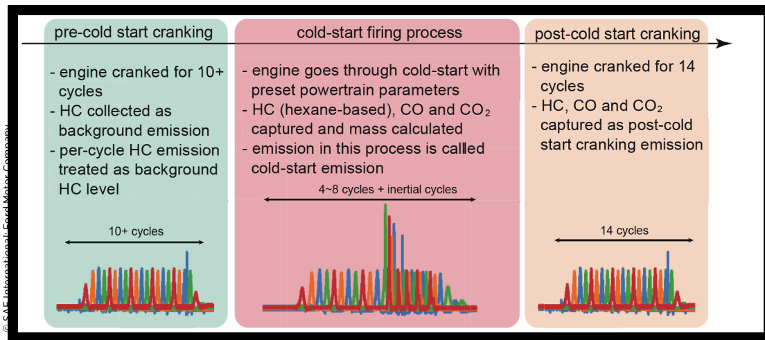
FIGURE 2 Experimental process
