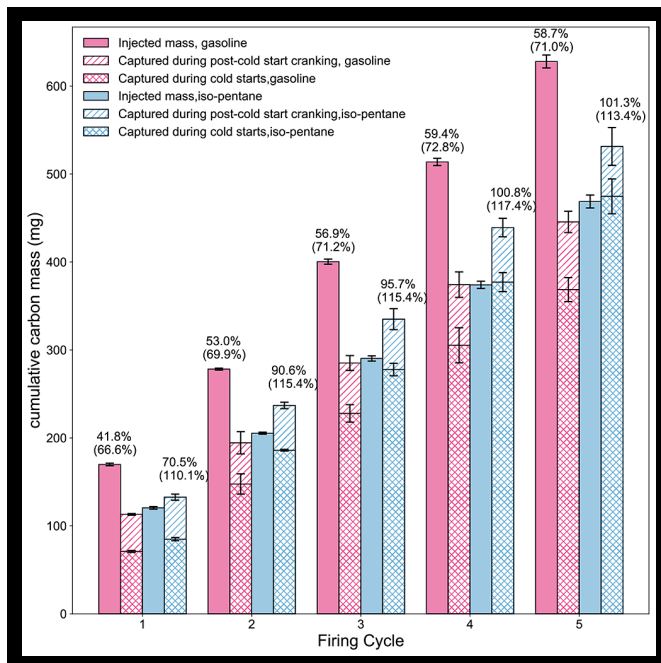
FIGURE 12 Cumulative carbon elemental mass injection and capture comparison
