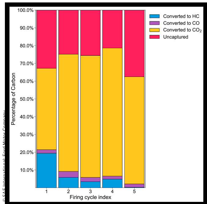
FIGURE 14 Percent carbon distribution for each individual firing cycle in the gasoline-fueled cold starts
