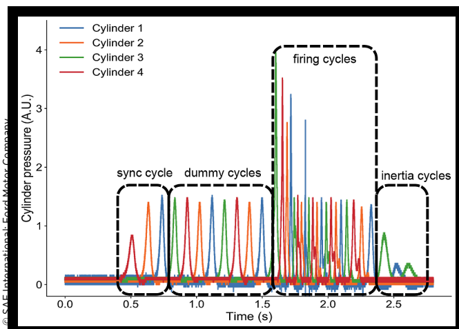
FIGURE 3 Cylinder pressure trace in a typical firing cold-start
