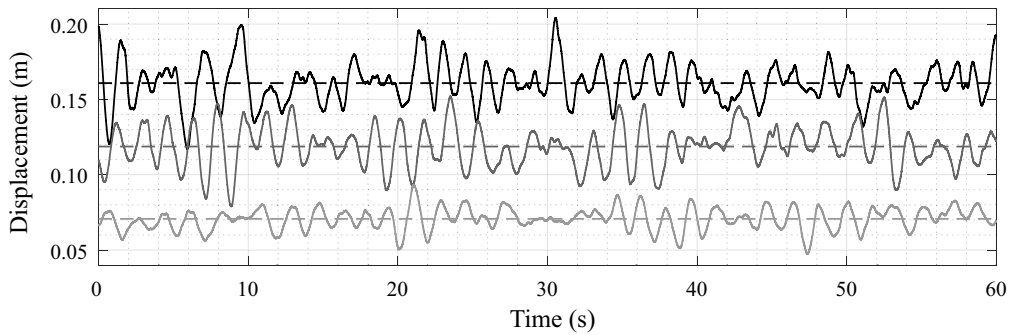
Figure 3. Examples of free end streamwise displacement vs. time over the 60 s steady-state periods for a PVC cylinder ( D = 3.8 \pm 0.1 cm) for U = [4.5, 5.6, 6.6] \pm 0.5 ms -1 (lines shaded from light to dark with increasing U ). Mean displacements are indicated with dashed lines. The observed streamwise oscillations are consistent with previous studies in steady flow (King, 1974).
