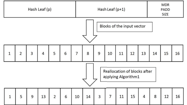
Figure 6: Mapping of SHA Input Blocks based on ECM.
