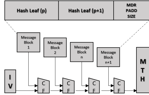
Figure 5: SHA256 for Merkle Tree Calculation
