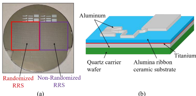
Fig. 3. (a) Prototype of the fabricated wafer and (b) unit cell depicting the RRS layered structure.
