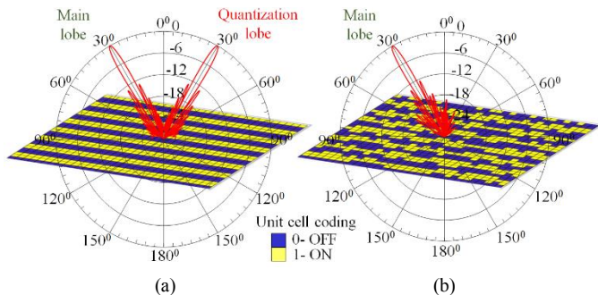
Fig. 2. 2D RRS with (a) 1-bit phase modulation results in a periodic phase distribution with an undesired quantization lobe (b) randomization perturbs the periodicity and the resultant radiation pattern consists of a single main lobe.
