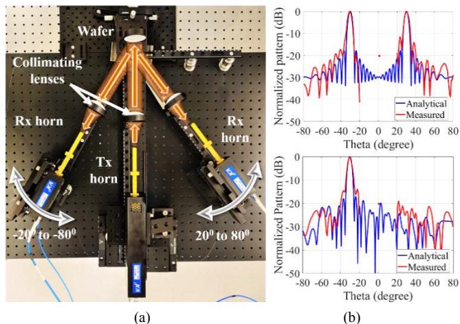
Fig. 4. (a) Quasi-optical measurement setup used for the characterization of the fabricated RRSs and (b) normalized RCS pattern v/s the scan angle theta at 222.5 GHz for non-randomized RRS (top) and randomized RRS (bottom).
