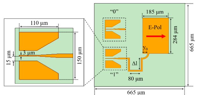
Fig. 1. A unit cell of the designed RRS.
