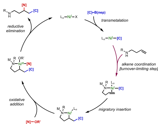
C. Proposed catalytic cycle
