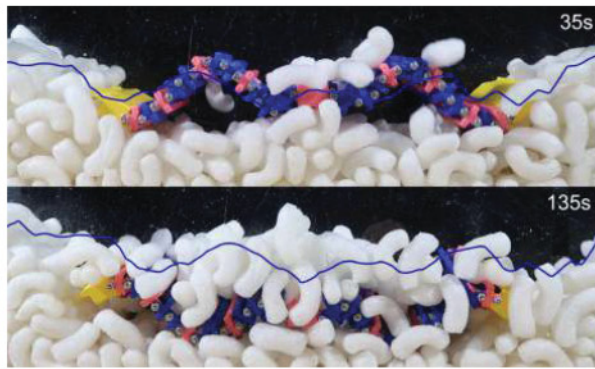
Fig. 5. Indentation and later submerging by an untethered robot, starting from a level surface (outline shown in blue).
