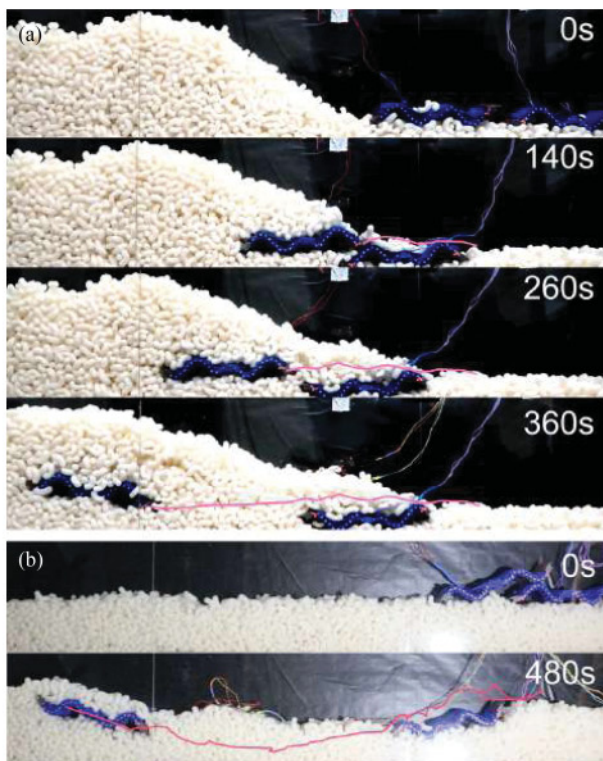
Fig. 8. Snapshots of collaborative burrowing sideways (a) and down (b) into granules; visually tracked path (smoothed over 15 s) of the burrowing robot is overlaid in pink.
