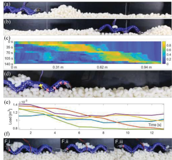
Fig. 6. (a)–(b) Snapshots before and after moving a mound. (c) Data from a single trial, showing the position of granules over time (the color denotes the fraction of image height per column in the frame, cropped just under the level surface). (d)–(e) Snapshot of a robot transporting granules and load volume over time. (f) Snapshots as robot stays in place while moving granules along the length of its body.
