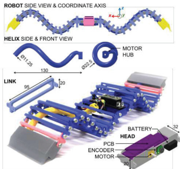
Fig. 2. Robot design. Dimension: 383 \times 62 \times 101 mm 3 . Weight: 283 g.
