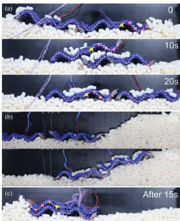
Fig. 7. (a) Two robots passing each other. (b) Robot helping another climb a 60% slope. (c) Stacked robots moving in synchrony accumulate material in their direction of motion.
