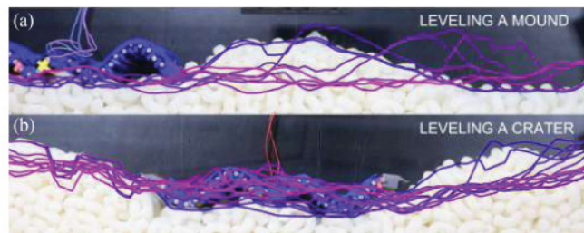
Fig. 4. Two leveling challenges, blue through pink curves show the granular surface over time. (a) The robot first pushes the mound right, then evens out the protrusion by moving back left. (b) The robot first levels out the right slope of the crater, then repeats the process on the left.
