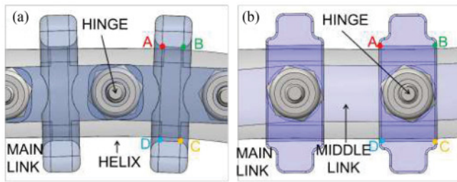
Fig. 9. (a) Present design, link on the helix. The helix progression rotates the link by forces at B and D or at A and C . Because hinges are not in the middle of the link, link interaction can cause moments. (b) Proposed link design, where 1) the contact distance, w , ( AB or CD ) has a larger moment on the link from a given normal contact force, and 2) buckling from compression in the chain is inhibited.
