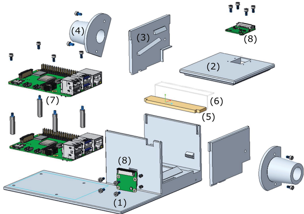
Fig. 2 Top: Exploded view of the entrance. Numbers relate to superscripts in the table below. The cameras are mounted ~55 mm from the tunnel surface. Note that all components are also available on Amazon, except for the 3D-printed pieces produced with PLA at 21.99 USD/kg. For assembly, users need a screwdriver, a box cutter, a needle nose plier, a soldering iron, a screen, and the ability to program the micro-SD cards
