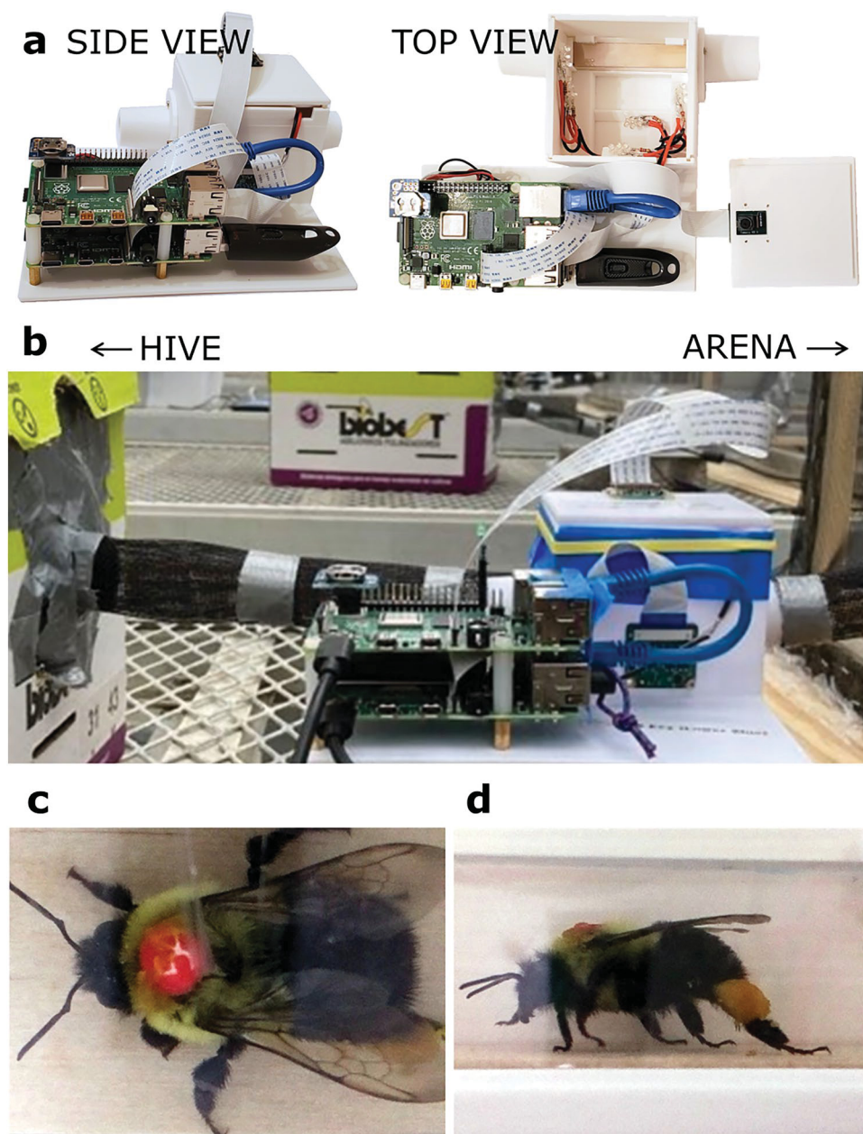
Fig. 1 Automated entrance monitor ( a , b ) capturing top and side photos ( c , d ) of bumble bees as they enter and exit their hive; the bee shown is carrying pollen. Note that to fit the format of this article, all photos from the cameras have been cropped
