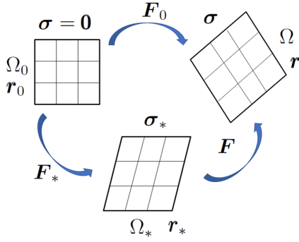
FIG. 1. The reference stress-free configuration \Omega_0 , the deformed (current) configuration \Omega under the Cauchy stress \sigma , and an arbitrary intermediate configuration \Omega_* with initial stress \sigma_* . The multiplicative decomposition of the deformation gradient \mathbf{F}_0 = \mathbf{F} \cdot \mathbf{F}_* is valid.
