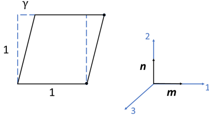
FIG. 2. Simple shear \mathbf{F} = \mathbf{I} + \gamma \mathbf{mn} with the shear strain \gamma at the plane with the unit normal \mathbf{n} along the unit direction \mathbf{m} . Crystal lattice of any symmetry can be oriented arbitrarily.
