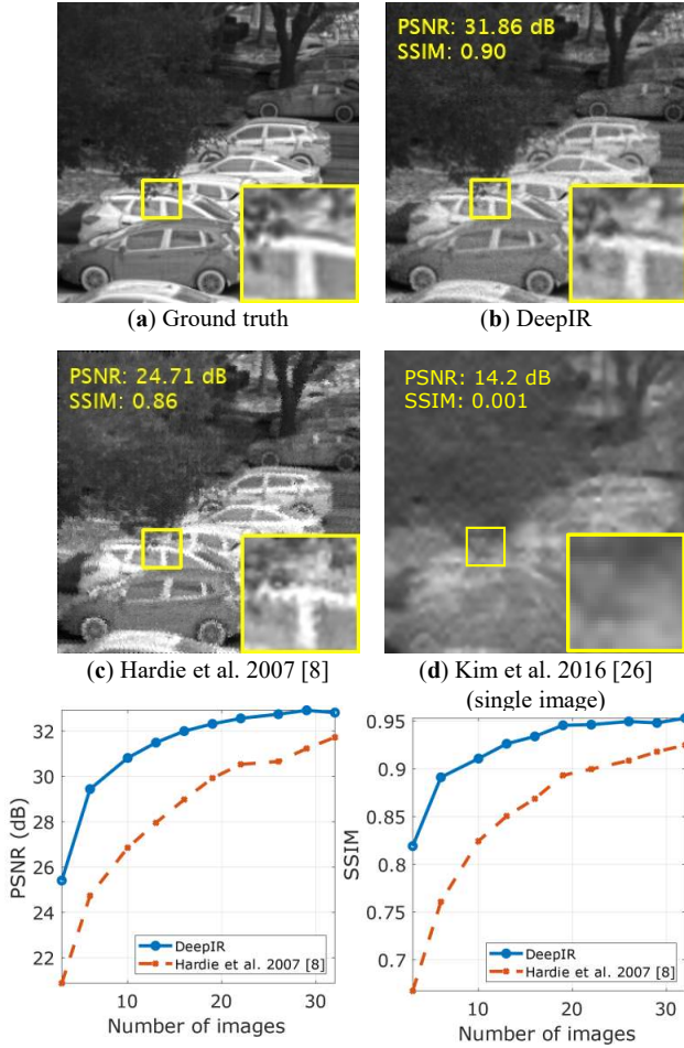
Figure 7: Simulations for super resolution. We simulated a capture of 16 images and performed a 4 \times super resolution with various approaches. DeepIR outperforms competing techniques including single image super resolution [26].
