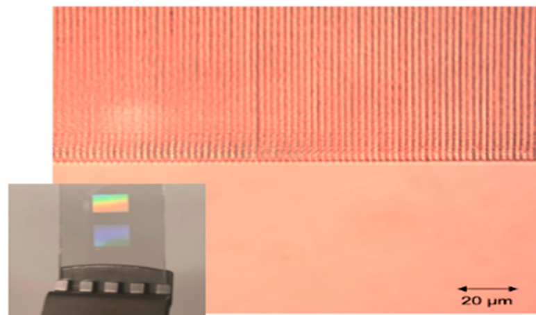
Figure 13. Femtosecond laser-induced Bragg structures in lithium niobate. Reprinted with permission from [48].
