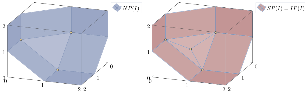
Fig. 2. The Newton, symbolic and irreducible polyhedra of I = (xy, xz, yz) .
