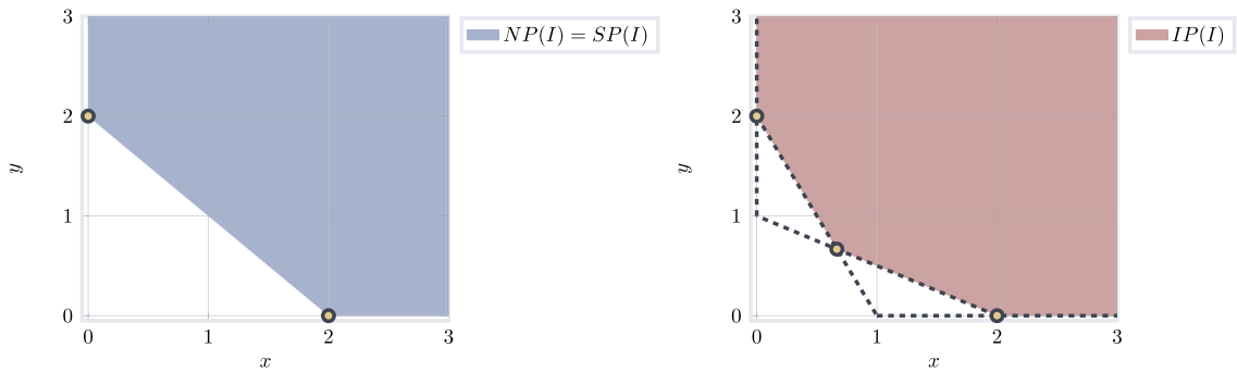
Fig. 1. The Newton, symbolic and irreducible polyhedra of I = (x^2, xy, y^2) .
