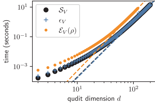
FIG. 2. Serial runtime to compute S_V , \epsilon_V , or \mathcal{E}_V(\rho) with |V| = 2d - 1 randomly chosen measurement axes and a randomly chosen qudit state \rho . Each point is an average over 10^3 calculations or 5 min of runtime, whichever comes first. These results do not count fixed runtimes to precompute quantities that can be recycled for every new choice of V and \rho . Dashed lines show fits to a runtime t = cd^\alpha for the 20 largest values of d , finding \alpha \approx 3.8 \pm 0.1 .
