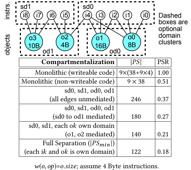
Figure 10: Privilege metric illustration.
