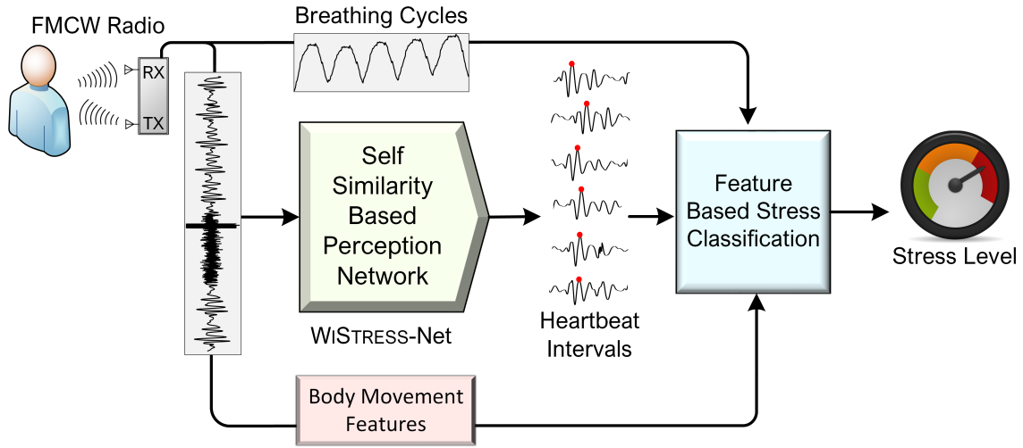
Fig. 2. Overview of WiStress's Design. The system uses a millimeter-wave FMCW radio to extract wireless reflections off the user's body. It filters these reflections to obtain time-domain signals that correspond to breathing cycles and micro-movements. The micro-movements are fed to a self-similarity-based perception network to extract individual heartbeats. Finally, the breathing cycles, heartbeats, and body movement features are fed into a stress classification network that infers a user's stress level.
