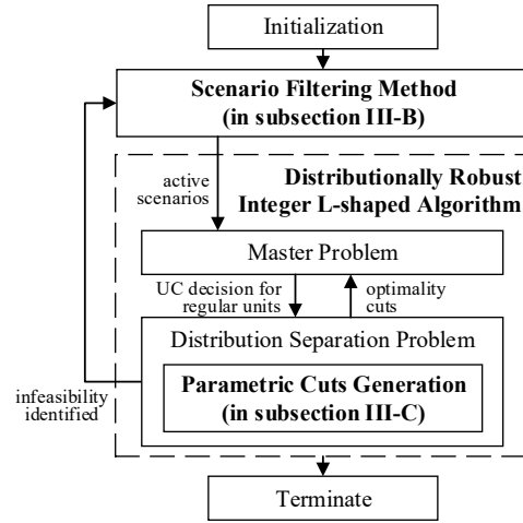
Fig. 1. Algorithmic framework.
