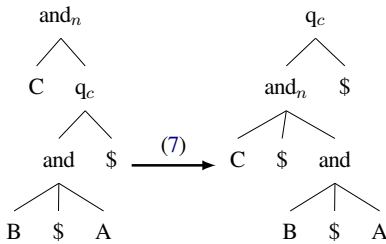
Figure 6: Application of rule (7) for flat prosody.
