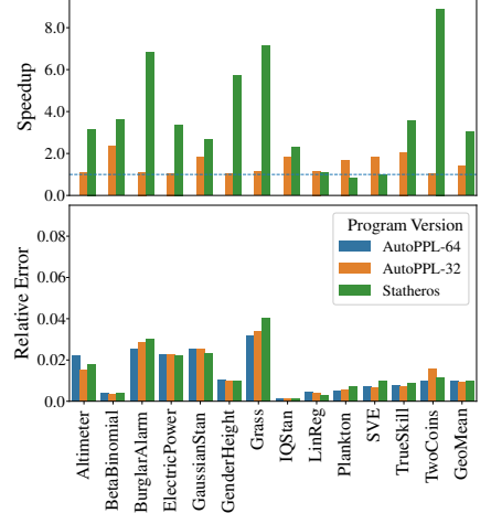
Fig. 4. Raspberry Pi Runtime and Accuracy
