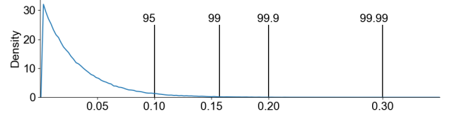
Figure 2: Estimated Tail Distribution (Exponential) and corresponding percentile estimates
