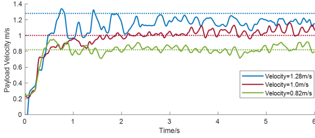
Fig. 7: Parameterized linear velocity tests. The commanded linear velocities used for tests are 0.82, 1.00, and 1.28 m/s (dashed lines). The actual velocity profiles are depicted in solid lines.
