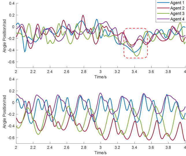
Fig. 8: Left front knee angles for four agents while traversing over challenging terrain. Top: Centralized policy results. Bottom: Decentralized policy results.
