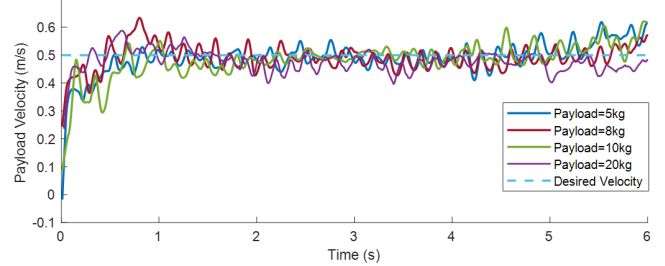
Fig. 6: Payload velocity tracking results on a 0.5 zScale terrain. The policy is trained with payload mass = 8 kg and tested with 5, 8, 10, and 20 kg.
