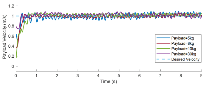
Fig. 4: Payload velocity tracking results of straight motion. The policy is trained with payload mass = 8 kg and tested with payload mass = 5, 8, 10, and 30 kg.
