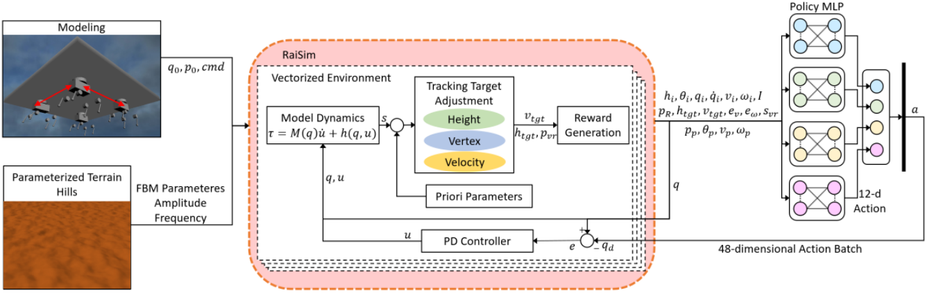
Fig. 2: Control architecture of collaborative quadrupedal manipulation. The initial agent parameter q_0 , terrain parameter p_0 and command cmd are the input of this architecture. System input p_0 describes the initial position of agents and payload, q_0 denotes initial joint configuration, and cmd is the linear velocity command for the payload. Prior parameters include p_{vi} in Eq. (2) and h_0, h_{tr} in Eq. (3). Our terrain is generated by Fractal Brownian Motion (FBM) and based on which, we tune the terrain curve’s amplitude and frequency. The model dynamics takes the robot’s generalized coordinates q and inputs u to produce the simulated state s . This is then used by the tracking target adjustment to generate target height h_{tgt} , vertex position p_{vr} and agent velocity v_{tgt} , which are used for the reward function. The decentralized MLPs obtain observation and rewards from the environment and each generates a 12-dimensional output, the desired joint positions. Adding up the 4 outputs gets a 48 dimensional action batch q_d . Then, a PD controller is utilized to convert desired joint positions to torques u .
