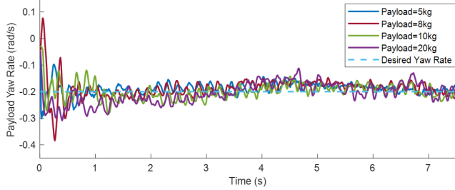
Fig. 5: Payload yaw rate tracking results of curve motion. The policy is trained with payload mass = 8 kg and tested with 5, 8, 10, and 20 kg.
