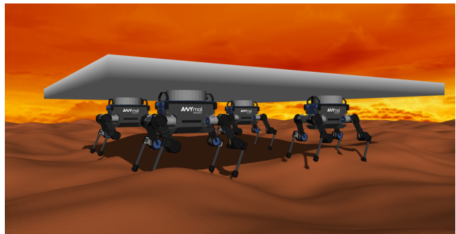
Fig. 1: Four quadrupeds traverse over challenging terrain at a desired velocity while collaboratively carrying a payload in RaiSim.
