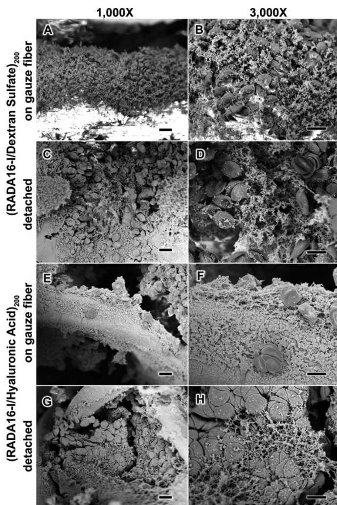
Figure 3 Surface characterization of anticoagulated whole blood upon contact with spray LbL assembled films. Scanning electron microscopy characterization of (RADA16-I/DS) 200 films ( a–d ) and (RADA16/HA) 200 films ( e–h ) in contact with anticoagulated whole blood shows that the blood components interact with the films both on the gauze fibers ( a, b, e, and f ) and once the films are detached from the gauze ( c, d, g, and h ). Figure adapted with permission from Reference 66, Copyright 2015, American Chemical Society. Abbreviations: DS, dextran sulfate; HA, hyaluronic acid; LbL, layer-by-layer; RADA16-I, RADARADARADARADA.
