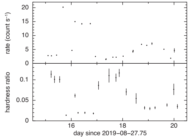
Figure 2. A zoom-in of the soft X-ray light curve and hardness ratio (2–10 keV/0.5–2 keV) from Fig. 1, but plotted in linear space to emphasize the variability. There is a clear anticorrelation between count rate and hardness.
