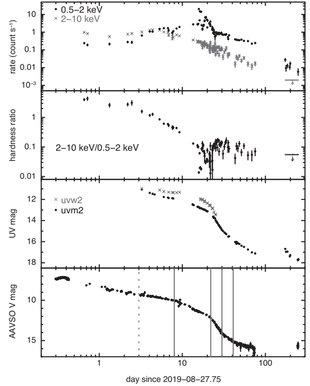
Figure 1. From top to bottom: Swift X-ray soft and hard band light curves, hardness ratio and UV light curves, and AAVSO V-band light curves. The vertical grey lines in the bottom panel mark the break times in the decay, as discussed in Section 6.3; the dotted line shows the time at which the parametrization of the UV/optical decay begins. Note that the final bins in the hard light curve and hardness ratio are upper limits.
