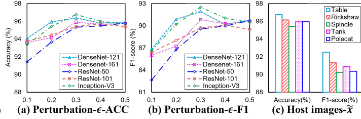
Figure 3: Evaluation with different \epsilon and host images \tilde{x} .
