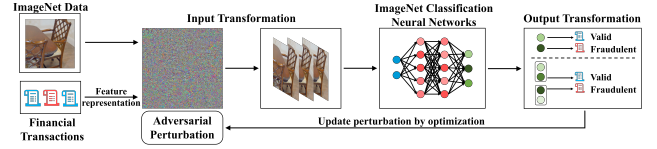
Figure 1: The overview of our proposed model AdvRFD.
