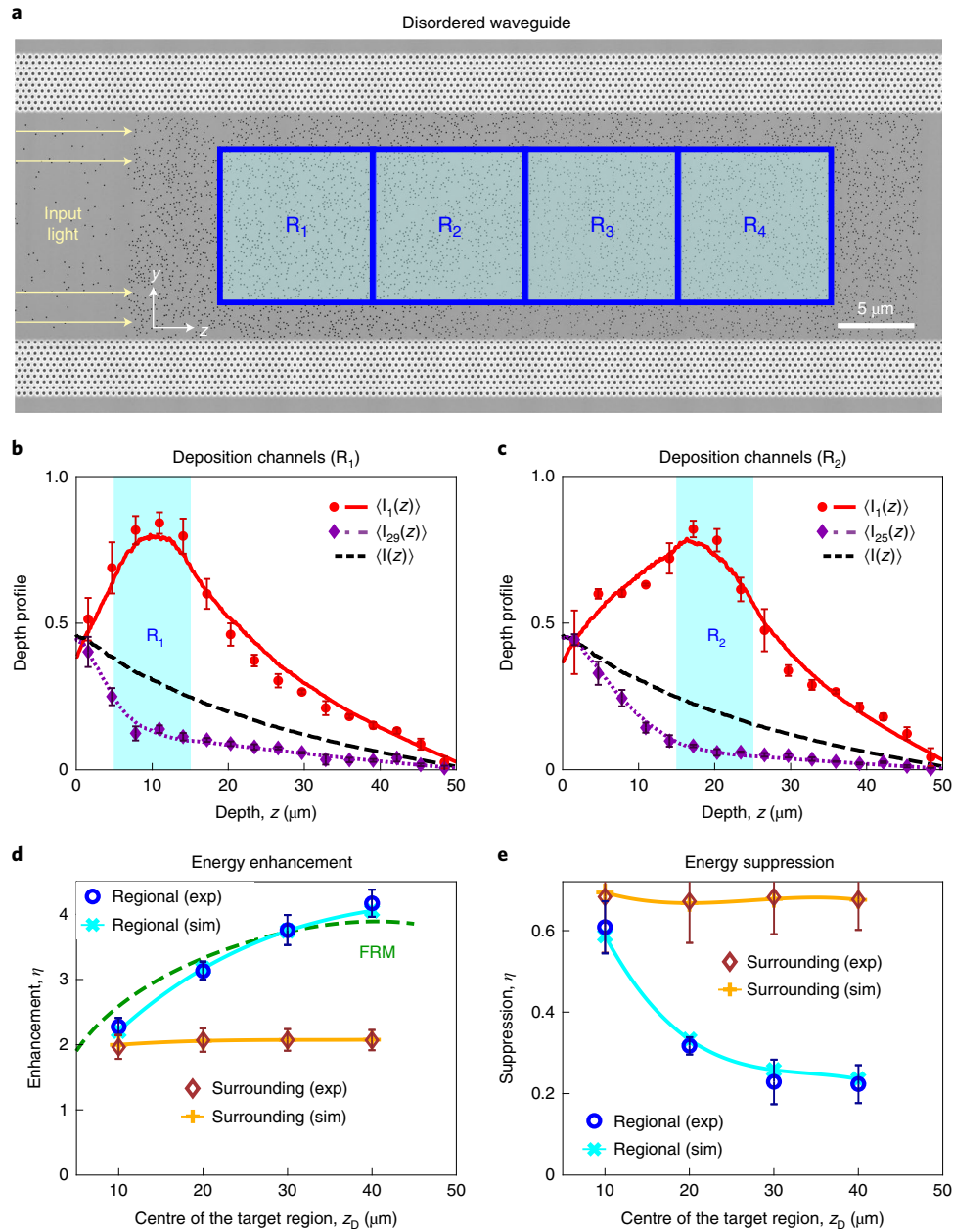
Fig. 3 | Experimental measurement of deposition eigenchannels. a , A composite scanning electron microscopy image of a disordered waveguide with width W = 15 \mu\text{m} . Randomly distributed air holes (each with a diameter of 100 \text{ nm} ) are etched throughout a designated 50\text{-}\mu\text{m} -long region. The four target regions used for energy deposition are superimposed; each is 10 \mu\text{m} \times 10 \mu\text{m} . b, c , Depth profiles (cross-section-integrated intensities) of two deposition eigenchannels with enhanced and suppressed energies in target region R_1 centred at depth z_D = 10 \mu\text{m} ( b ) and R_2 at z_D = 20 \mu\text{m} ( c ). The experimentally obtained data for the cross-section-integrated intensity (red circle and purple diamond) agrees with the numerical simulations (red solid line and purple dotted line), and the normalized root-mean-square difference values between the measured and simulated eigenchannels are as follows: 0.10 for \alpha = 1 and 0.13 for \alpha = 29 ( b ); 0.08 for \alpha = 1 and 0.09 for \alpha = 25 ( c ). The black dashed line is the intensity profile averaged over random input wavefronts. Each experimental data point is averaged over \Delta z = \ell , and the error bar corresponds to \pm one standard deviation. d, e , Experimentally measured energy enhancement in the target region \eta_t (blue circles) and surrounding area \eta_s (brown diamonds) of two deposition eigenchannels \alpha = 2 ( d ) and \alpha = 24 ( e ) are compared with the numerical data (light-blue and orange lines; denoted as ‘sim’) for the case of energy deposition into the four target regions centred at 10, 20, 30 and 40 \mu\text{m} . The theoretically predicted maximum energy enhancement, including loss and incomplete channel control (green dashed line in d ), agrees with the experimental (exp)/numerical results, confirming the essential contribution of long-range intensity correlations to energy deposition.
